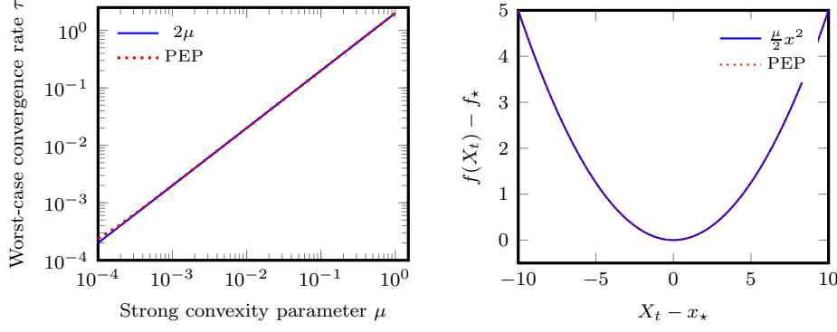
(a) Worst-case rate \tau_* for the class of quadratic Lyapunov functions (2.2) (b) Reconstruction of a function f \in \mathcal{F}_{\mu, \infty} that interpolates x_* and X_t , while matching the convergence rate \tau_* = 2\mu , with \mu = 0.1 .
