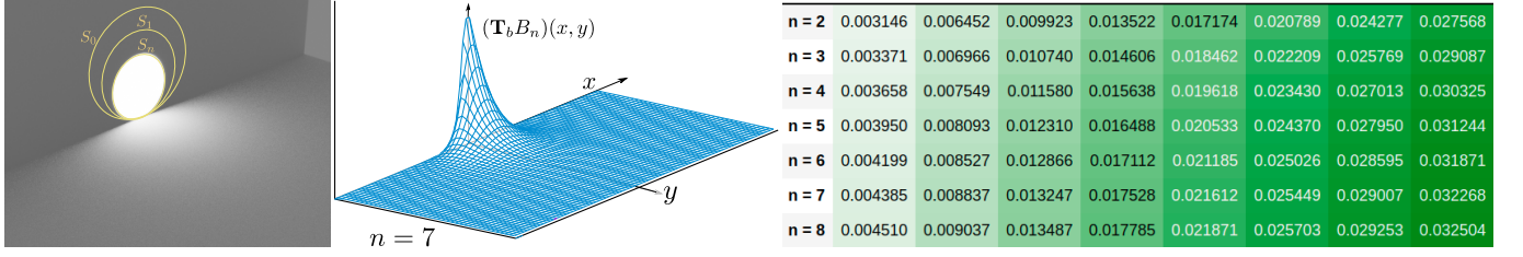
Fig. 3. Illustration of our proof that the radiant exitance transport operator \mathbf{T}_b is not compact. Left : rendered scene with a disk S_n emitting diffuse light. The disk is tangential to the abutting edge. Center : measured radiant exitance on the receiver surface for n = 7 . As n is increased, the spatial frequencies of the emitted energy increases while preserving its L_2 norm, as does the received energy. In the limit, it escapes any finite rank approximation over the space of functions on the receiver. Right : table showing that the pairwise measured L_2 distances between \mathbf{T}_b B_n and \mathbf{T}_b B_{n+p} do not depend on n (for large n , because the receiver is bounded) and converges to non-zero values with p for a given n . To ensure numerical accuracy in this figure we reduce the disk radius by a factor of 1.2 instead of 2, and use the analytical formula of Naraghi [1988].
