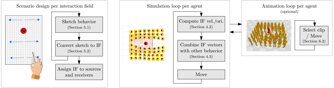
Figure 2: Outline of a complete simulation system with interaction fields. See Section 3 for a textual overview.
