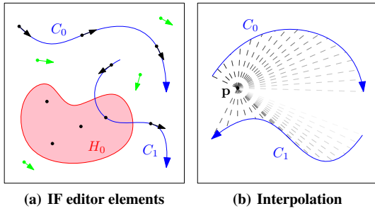
Figure 5: Concepts of the IF editor. (a) The user can draw guide curves (blue) and zero areas (red) to specify IF vectors; example vectors are shown in black. IF vectors for points in-between will be interpolated (green). (b) For any point p outside all zero areas, the IF vector is a weighted average of all vectors along all guide curves, where weights depend on the distance to p .
