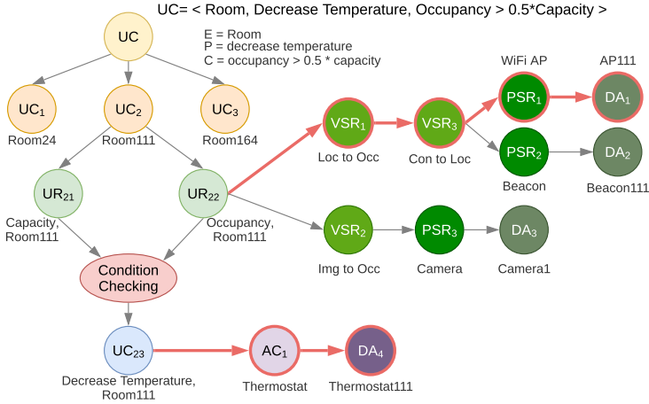
Fig. 12. Example of the translation of a user command.
