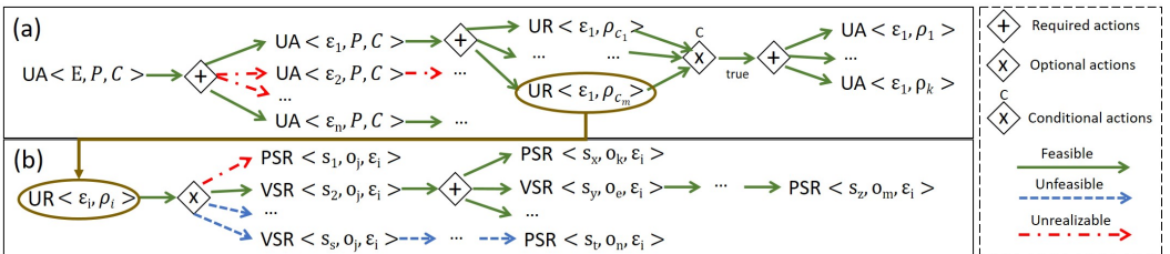
Fig. 11. Structures generated to handle a User Action: (a) Flattened tree for UA and (b) Execution plans generated for a UR .
