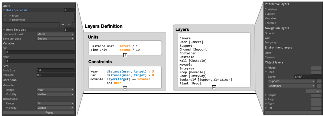
Fig. 7. Schema of the layers definition interface, which allows the designer to add and edit the units, constraints, and layers either through point-and-click or importing a configuration file. The Unity interface is shown on the two sides.
