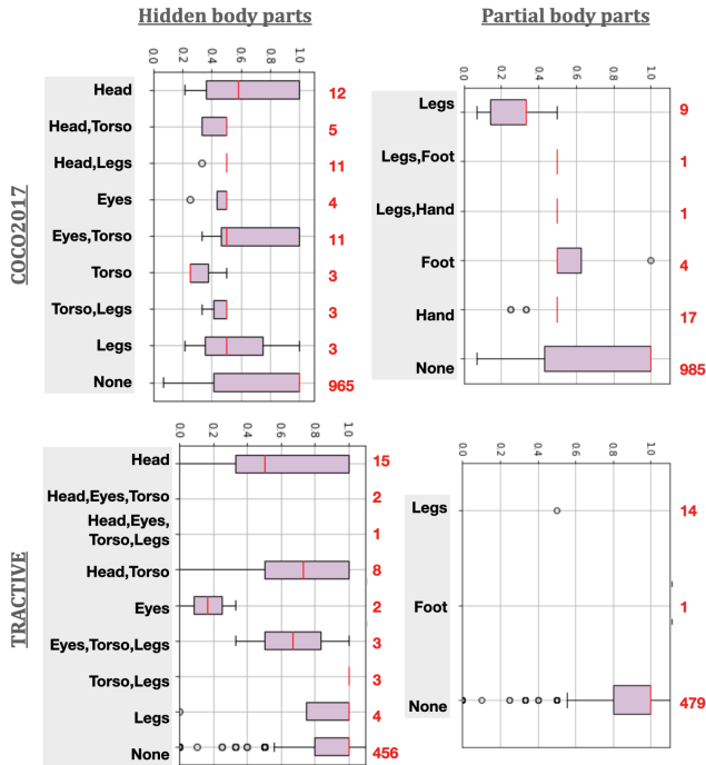
Figure 6: Boxplot of recall per image, images grouped by hidden (left) and visible (right) body parts. Figure shows that missed detections are almost systematic when only headless body parts are visible (right column).
