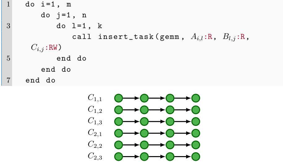
Figure 5: Parallel GEMM using the baseline STF model. A generated DAG is proposed with m = 2, n = 3, k = 4 with green circles representing GEMM tasks. Each chain of tasks in the DAG corresponds to contributions to a single block.
