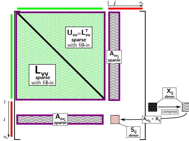
FIGURE 8: Computation loop of S in compressed Schur multi-factorization . Compressed matrices are represented with corrugated background. Constructing W requires a temporary deduplicated storage of A_{vv} , A_{sv_i} , A_{sv_j}^T .
