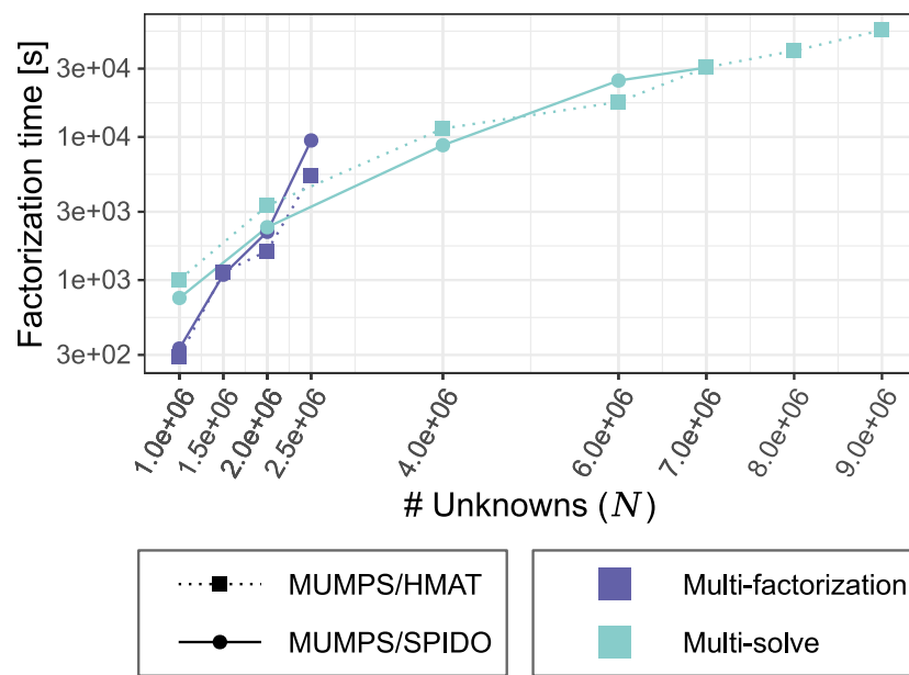
FIGURE 10: Best computation times of multi-solve and multi-factorization for both of the solver couplings MUMPS/HMAT and MUMPS/SPIDO. Parallel runs using 24 threads on single miriel node.
