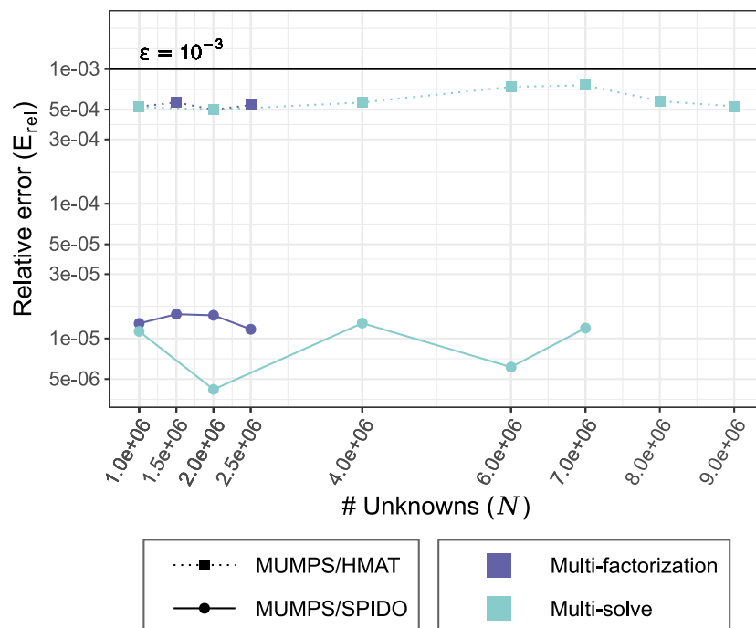
FIGURE 11: Relative error E_{rel} for the runs of multi-solve and multi-factorization having the best execution times and for both of the solver couplings MUMPS/HMAT and MUMPS/SPIDO. Parallel runs using 24 threads on single miriel node.
