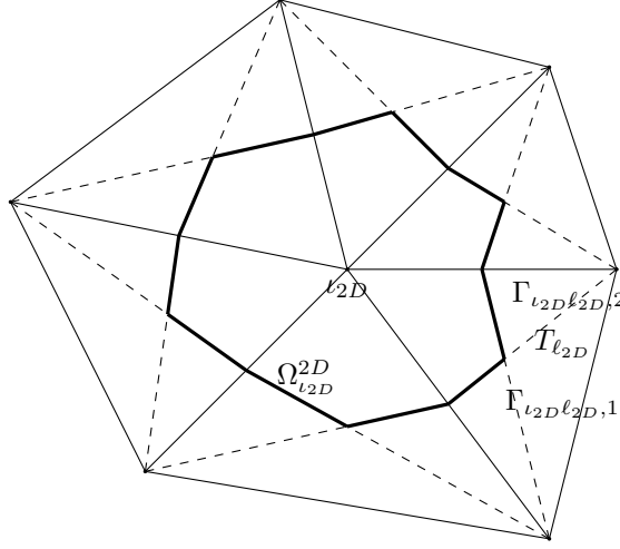
FIGURE 1. Representation of a control cell \Omega_{\ell_{2D}}^{2D} in the (R, Z) -plane.
