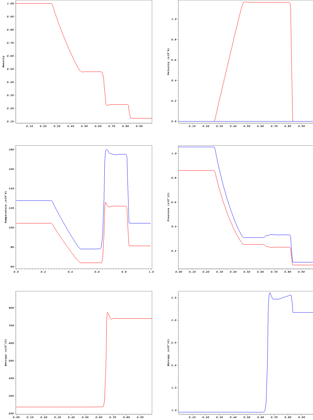
FIGURE 3. Shock tube problem at t = 8.6289 \times 10^{-8} s with \nu_{ei}^e = 0 . Solution at y = 0.5 . Left-Top: Density, Right-Top: x -velocity in red, and y -velocity in blue, Left-Center: Electron (red) and ion (blue) temperatures, Right-Center: Electron (red) and ion (blue) pressures, Left-Bottom: Electron entropy, Right-Bottom: Ion entropy.
