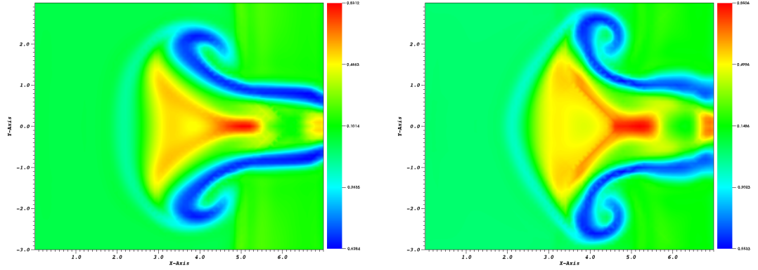
FIGURE 17. Triple point problem, \frac{T_i - T_e}{T_e} 2D field at t = 3.5 s (Left), and t = 5.0 s (Right).
