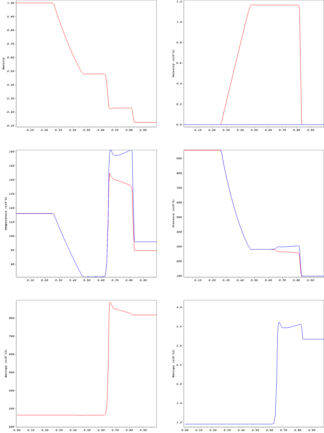
FIGURE 4. Shock tube problem at t = 8.6289 \times 10^{-8} s with \nu_{ei}^e \neq 0 . Solution at y = 0.5 . Left-Top: Density, Right-Top: x -velocity in red, and y -velocity in blue, Left-Center: Electron (red) and ion (blue) temperatures, Right-Center: Electron (red) and ion (blue) pressures, Left-Bottom: Electron entropy, Right-Bottom: Ion entropy.
