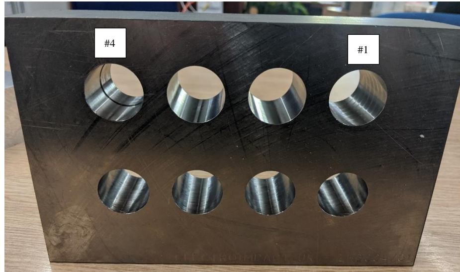
Fig. 6. Production Cutter Coupon Drill and Ream Holes (Holes 1,2,3: One-Shot Drill 27.5mm & Ream 28.5mm, Hole 4: Partial Ream, Holes 5,6,7,8: One-Shot Drill 27.5mm)
