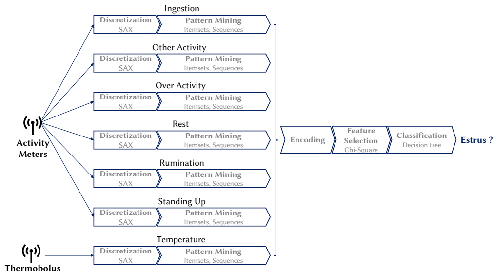
Figure 1: Pipeline of the pattern-based classifier XPM.
