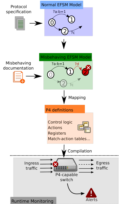
Fig. 1: Approach overview
