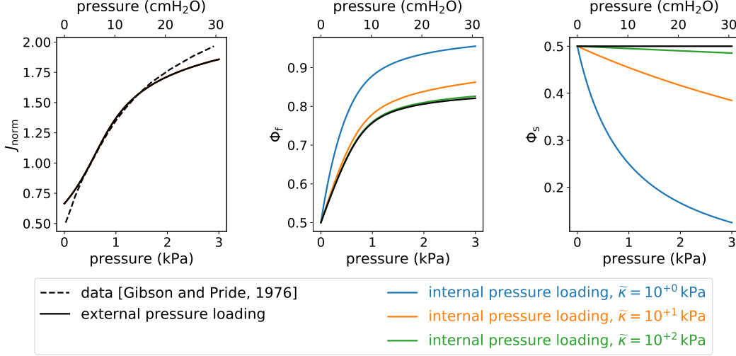
Figure 2: Mechanical response of the mixture resulting from our choice of \widetilde{W}_{\text{skel}} in Eq. (27) & \widetilde{W}_{\text{bulk}} in Eq. (29) for various values of bulk modulus \bar{\kappa} (while other parameters are fixed at \Phi_{f0} = 0.5 , \bar{\alpha} = 0.16 kPa, \bar{\beta}_1 = 0.2 kPa, \bar{\beta}_2 = 0.4 kPa & \delta = 0.5 ) and applied pressure – positive when internal or negative when external, here considered in absolute value in the plots. The solid black curve corresponds to an external negative pressure loading ( i.e. , by imposing \underline{\Sigma} > 0 and p_f = 0 , in which case the response only depends on \widetilde{W}_{\text{skel}} , not \widetilde{W}_{\text{bulk}} , hence not on \bar{\kappa} ), while the colored curves correspond to a positive internal pressure loading ( i.e. , by imposing p_f > 0 and \underline{\Sigma} = 0 , in which case the response depends on \bar{\kappa} , so various values are considered). All curves are obtained by imposing a level of pressure and solving the nonlinear behavior law at one single material point – i.e. , a Rivlin cube – through a Newton-Raphson procedure, in order to compute the associated mixture deformation & volumes fractions changes. (Left) Volumetric response of a mixture to a pressure loading, compared to experimental data [Gibson and Pride, 1976]. J_{\text{norm}} is the mixture volume change J normalized by its value at 0.5 kPa (which roughly corresponds to the end-exhalation state in the lung model), leading to J_{\text{norm}} = J/J_{0.5} = 1 for an applied pressure of 0.5 kPa. The colored curves are superimposed with the black curve because the mixture volume deformation is identical for internal vs. external applied pressure. (Center & Right) Evolution of the volume fraction of fluid ( i.e. , the porosity) and solid with the pressure loading. When the mixture is subjected to internal pressure, the solid phase is compressed according to its bulk modulus; the lower the bulk modulus, the more compressible the solid, the higher the volume fraction of fluid and the lower the volume fraction of solid. For the value of the bulk modulus used in the rest of the paper ( \bar{\kappa} = 10^2 kPa) the change in solid volume is very limited.
