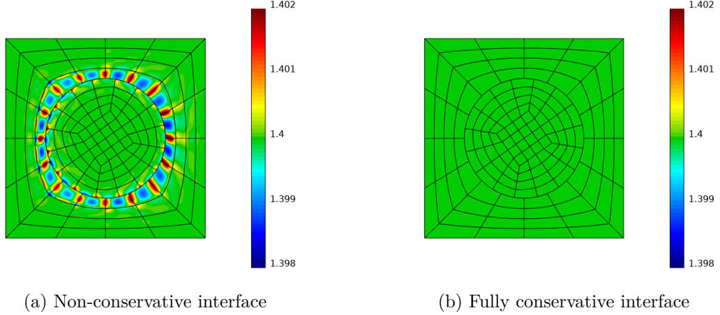
Figure 4: Freestream preservation with non-conservative and conservative sliding interfaces
