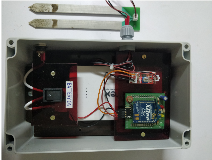
Fig. 2. Mote Connected with Soil Moisture Sensor
