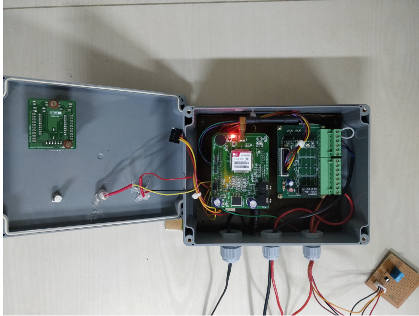
Fig. 4. Gateway Comprising GSM Module
