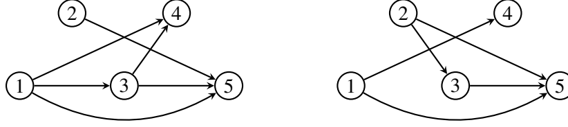
Figure 3: The dependency graphs for the two examples of Fig. 2; the left and right graphs correspond respectively to the single- and multi-agent examples presented therein. The active feedback at time t is exactly the set of in-neighbors of the corresponding vertex.
