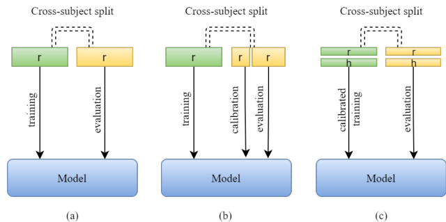
Figure 1: Different types of gaze estimation methods: (a) person-independent technique, (b) person-specific technique, (c) FLAME. Training subjects are green and test subjects are yellow. r stands for RGB image and h stands for eye landmark heatmap.
