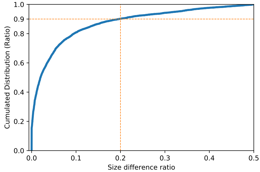
Figure 13: Cumulative Distribution of ratios between two versions of web pages. The orange dotted lines show the threshold used in this experiment
