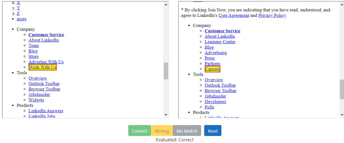
Figure 7: Labeling a given element matched by ERRATUM on two versions of the LinkedIn homepage. The screenshot comes from the visual matching application we created to manually label disagreements between ERRATUM & WATER.
