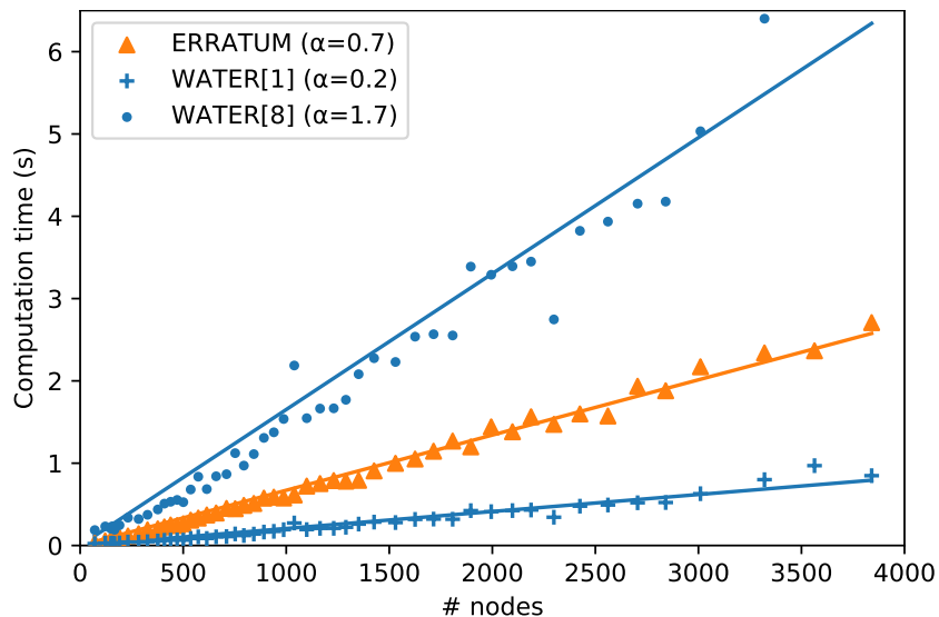
Figure 16: Repair time evolution according to DOM size.
