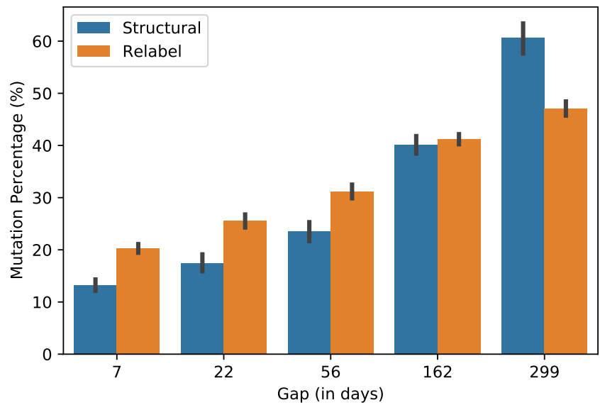
Figure 14: Mutation ratio between two WAYBACK snapshots depending on gap duration.
