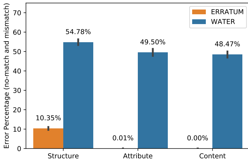
Figure 9: Error percentage according to the mutation type.
