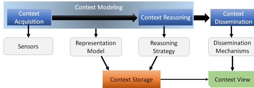
Fig. 1. Steps involved to obtain the context awareness.
