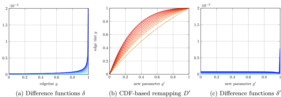
Figure 3: Reparametrization of the complex refractive index. (a) When using Gulbrandsen’s parametrization, material differences \delta along the edge tint dimension g for various reflectivities r exhibit a strong increase toward g = 1 . (b) Our CDF-based approach provides a mapping from a new edge tint parameter g' to Gulbrandsen’s edge tint g . The dashed curves show the rational polynomial fits we obtain. (c) After remapping, the difference functions \delta' are close to constant throughout the g' dimension. The only exception occurs for very high r and g' where the fit slightly loses its accuracy, which we have found sufficient in practice though.
