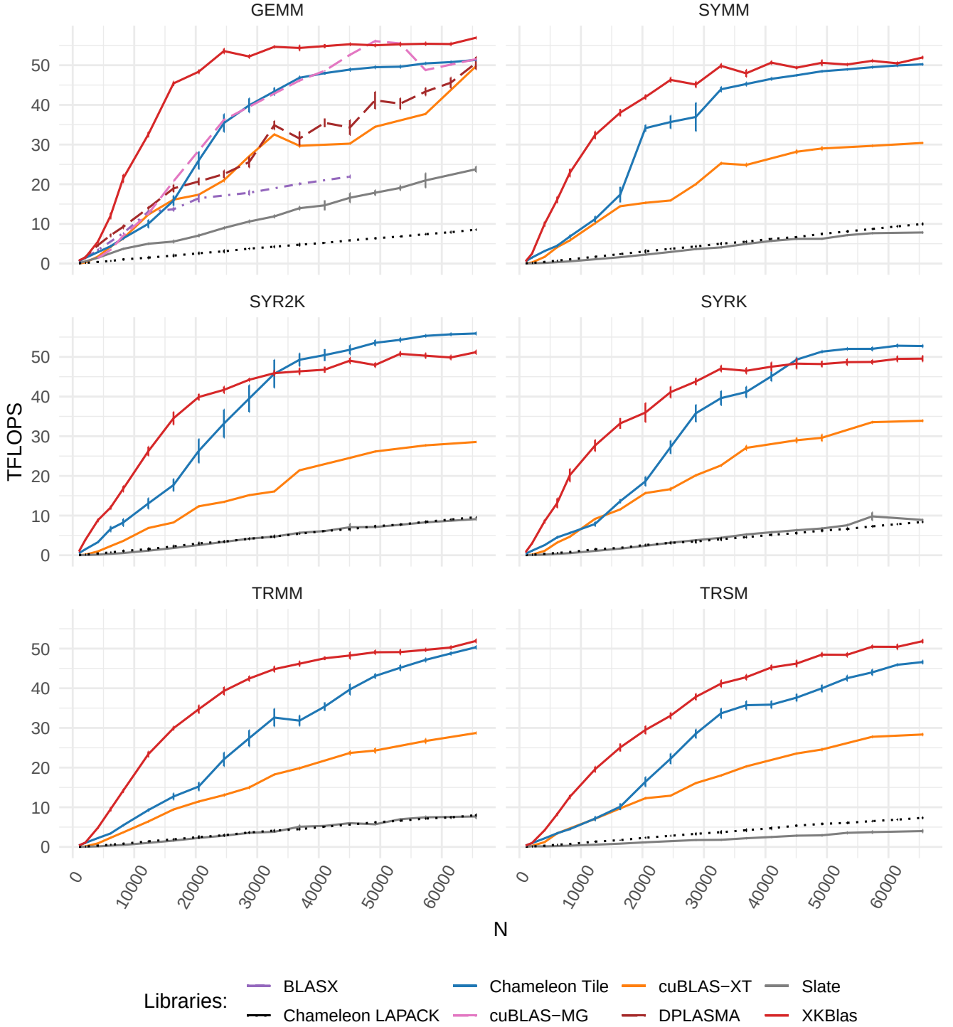
Fig. 5. Performance of libraries on DGX-1 with 8 GPUs for 6 BLAS subroutines. Chameleon LAPACK (black dotted line type) reports performance when input and output matrices are stored using LAPACK layout, while Chameleon Tile uses tile representation. BLASX DGEMM reports memory allocation errors when running with bigger matrices than 45 000. Error bars display the 95% confident interval of each point.
