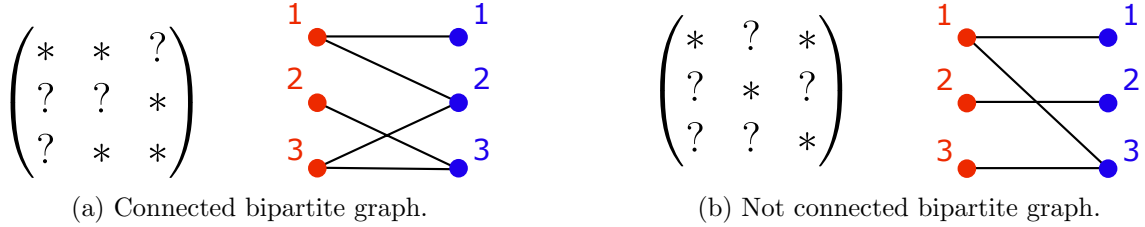
Figure 2: Illustration of Proposition 4.18: on the left, it is possible to complete the missing values denoted by “?” from the nonzero observed values “*” in the mask, because the bipartite graph associated to this mask is connected. On the right, this condition is not verified.
