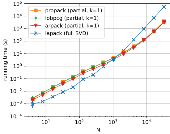
(a) Unbalanced tree, matrix of size N \times N
