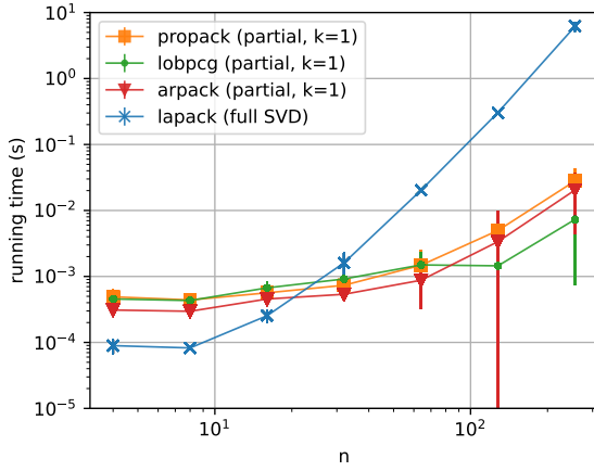
(c) SVD for matrices of size 2 \times n^2/2
