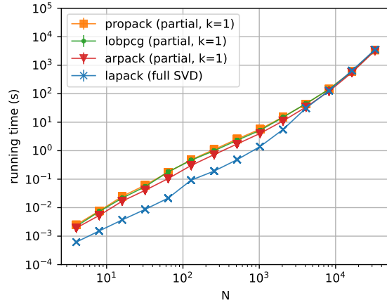
(b) Balanced tree, matrix of size N \times N
