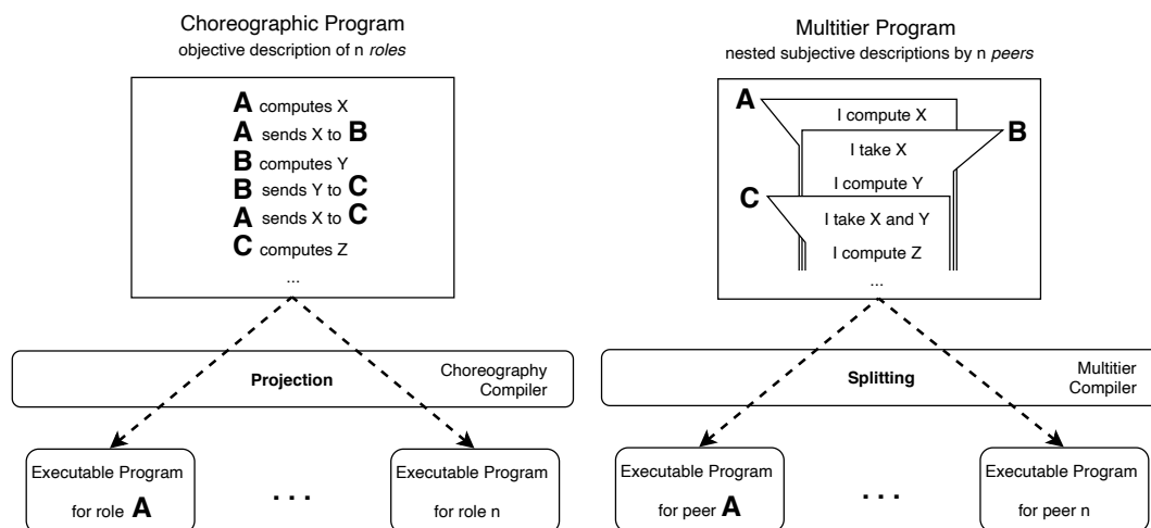
■ Figure 1 Choreographic Programming.
