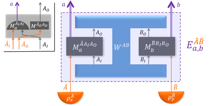
FIG. 1. SDI-QI scenario (main): A process matrix W^{AB} connects two parties who receive quantum inputs \rho_x^{\tilde{A}} and \rho_y^{\tilde{B}} , resp. They each perform a joint operation ((M_a^{\tilde{A}A I A O})_a and (M_b^{\tilde{B}B I B O})_b , resp.), and produce the classical outcomes a and b . The purple box shows the D-POVM (E_{a,b}^{\tilde{A}\tilde{B}})_{a,b} induced by these instruments and the process matrix. Inset: In the MDCI scenario (see later), additional structure is assumed on the quantum instruments (shown here for Alice). The quantum input is a bipartite state in \mathcal{H}^{\tilde{A}I\tilde{A}O} , a measurement is performed jointly on \mathcal{H}^{\tilde{A}I\tilde{A}I} and a channel sends \mathcal{H}^{\tilde{A}O} to the process matrix through \mathcal{H}^{A O} .
