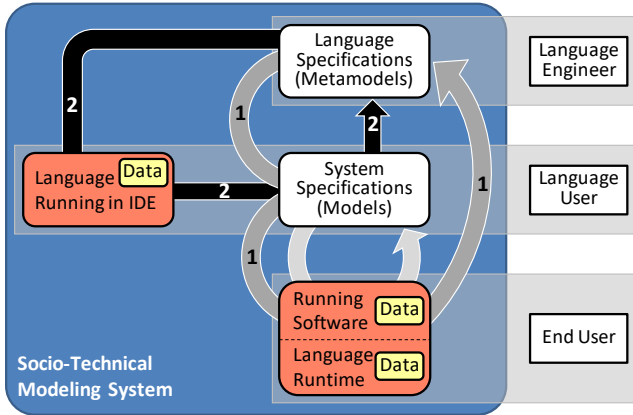
Figure 1. L-MODA Reference Framework for Self-Adaptable Languages
