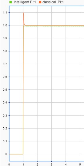
(a) Simulated results on the relationship between Classical PI and the intelligent P based on the relational gains
