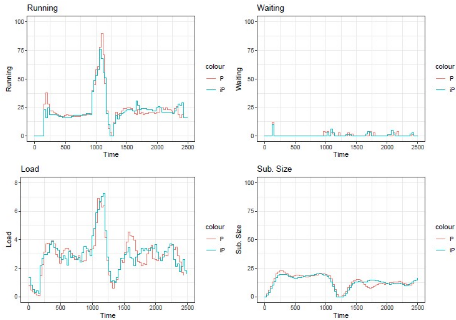
Fig. 10. Comparative Simulation results on the Grid'5000 between an Intelligent P and a classical P with local users
