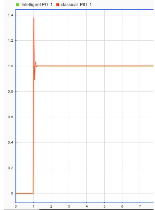
(b) Simulated results on the relationship between Classical PID and the intelligent PD based on the relational gains
