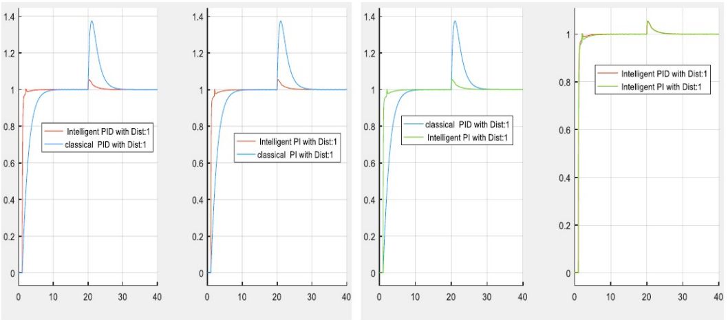
Fig. 6. Comparative Simulation results on a first order Plant with disturbance
