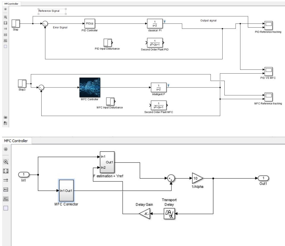
Fig. 13. The MFC Simulink blocks
