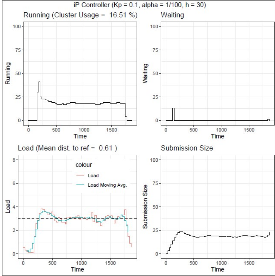
Fig. 11. Simulation results on the Grid'5000 using an Intelligent P based on cluster usage
