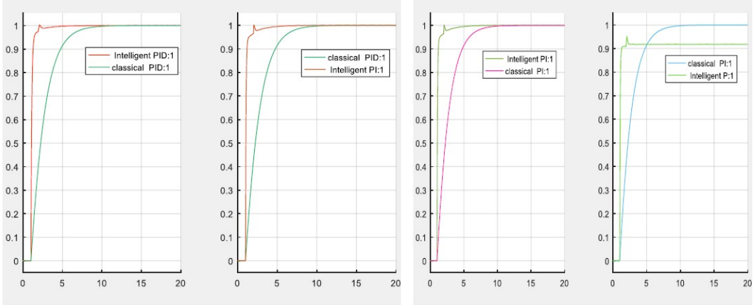
Fig. 5. Comparative Simulation results on a first order Plant without disturbance
