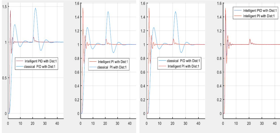
Fig. 8. Comparative Simulation results on a Second order Plant with disturbance
