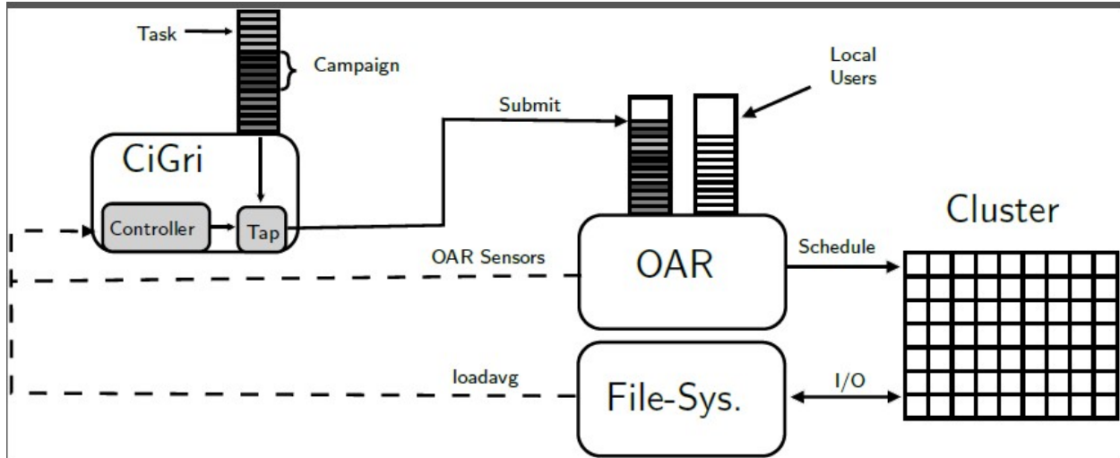
Fig. 3. A schematic overview of our cluster workflow
