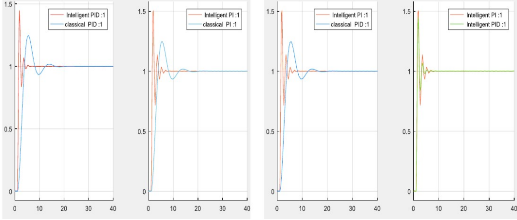
Fig. 7. Comparative Simulation results on a Second order Plant without disturbance
