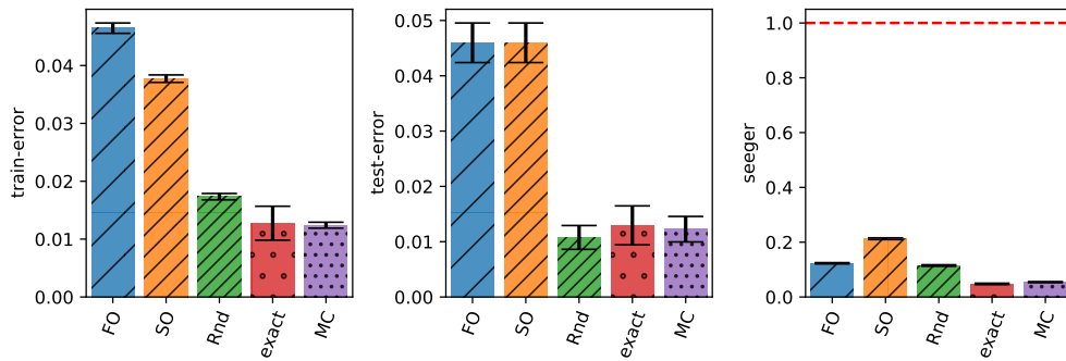
MUSHROOMS: d=22, n=6499
