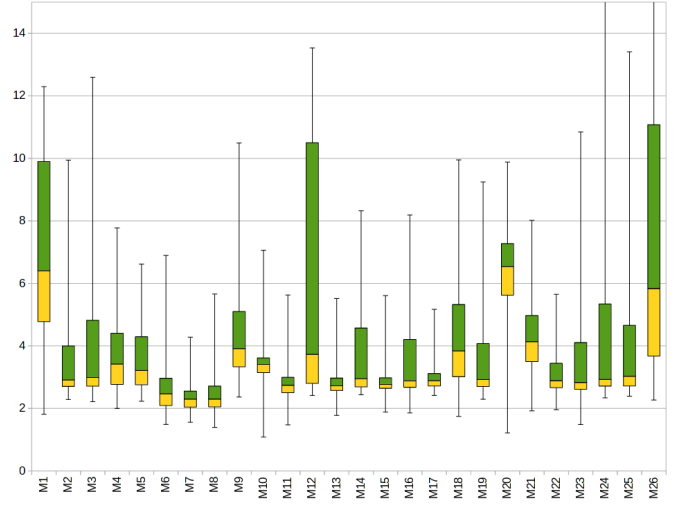
(b) Energy consumption per movement feature.
