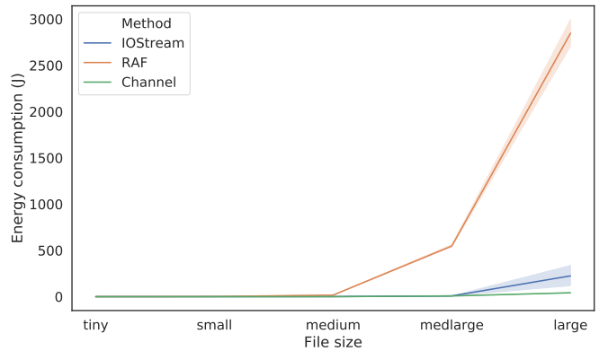
Fig. 6: Energy consumption to seek data from files of different sizes.
