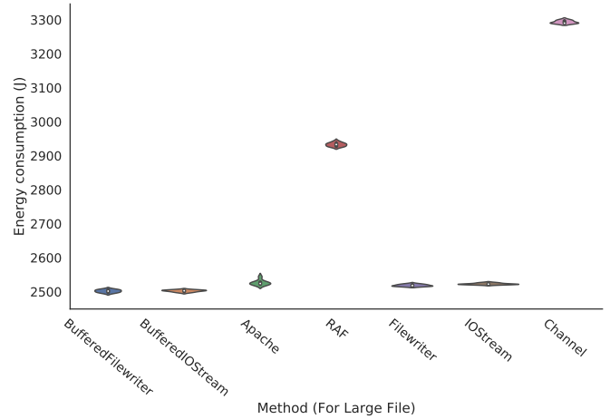
Fig. 8: Energy consumption of write methods for a large file.
