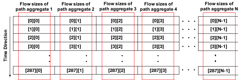
Fig. 8. The structure of observed matrix of aggregated flow size.
