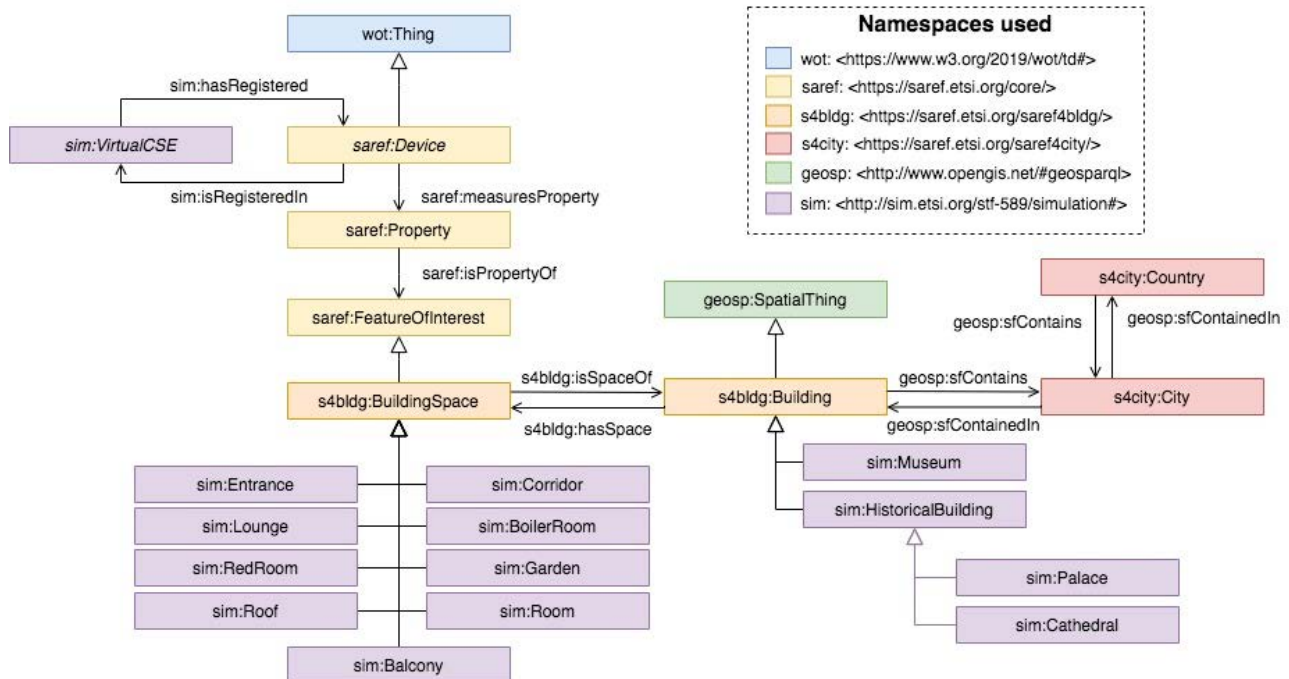
Figure 6.2.0-1: DSRD Ontology
