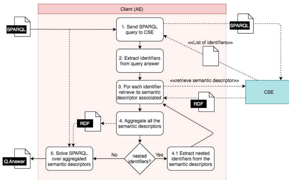
Figure 6.7.1-2: Workflow to be implemented to answer a SPARQL query by means of the current oneM2M Semantic Resource Discovery
