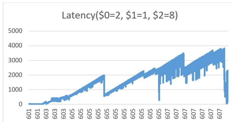
Figure 5.4.2-4: Latency ($0=2, $1=1, $2=8)
