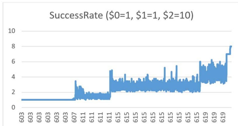
Figure 5.4.3-2: Success Rate ($0=1, $1=1, $2=10)
