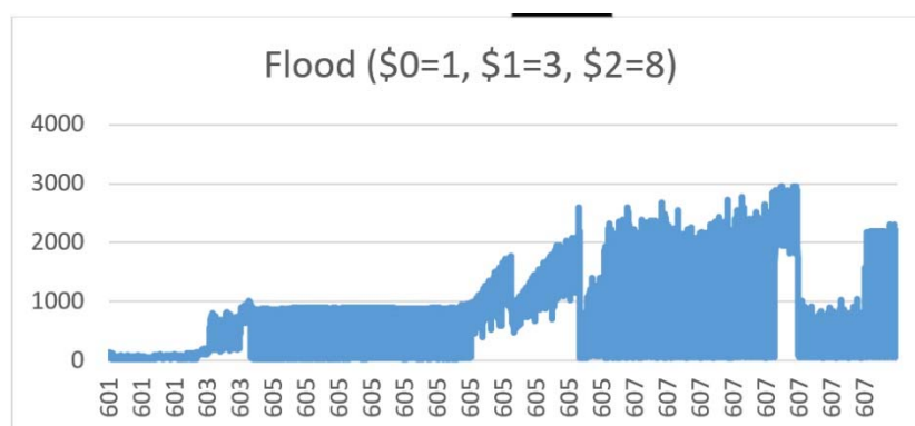
Figure 5.4.4-3: Flood ( \$0=1 , \$1=3 , \$2=8 )
