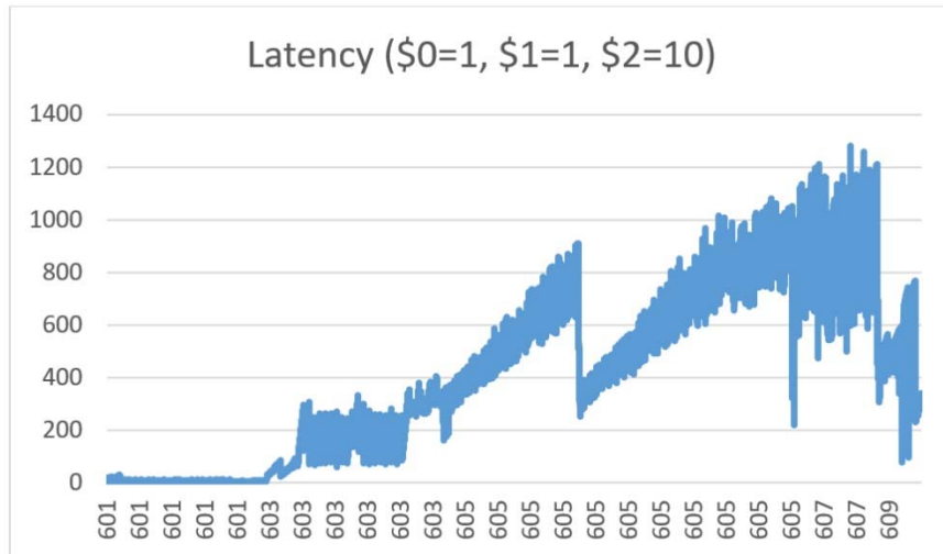
Figure 5.4.2-2: Latency ($0=1, $1=1, $2=10)
