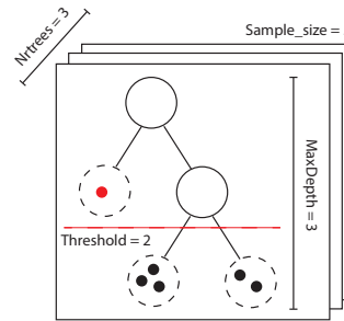
Fig. 3. Parameters in isolation forests manipulate the forest by specifying the number of trees, number of nodes per tree, the maximum depth of generated trees along with the number of samples that must be used for the construction of a tree. The dot in red is anomalous with respect to the chosen threshold.
