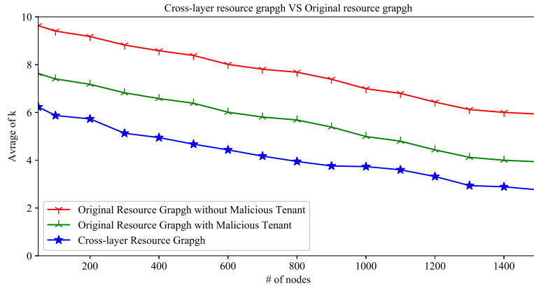
Fig. 5: Comparing the original resource graph and cross-layer resource graph
