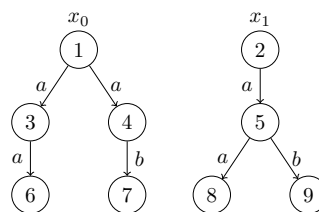
Fig. 1: Spoiler has a winning strategy at (x_0, x_1) .
