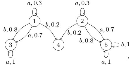
Fig. 4: Probabilistic transition system
