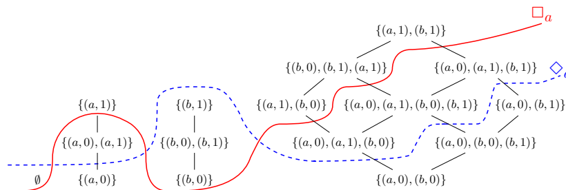
Fig. 2: The set F2 = \mathcal{P}_f(\{a, b\} \times 2) with the order \leq^F (for labelled transition systems). The modality \square_a ( \diamond_a ) is given by the elements above the solid (dashed) line.
