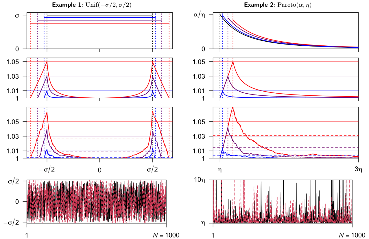
FIG 1. Illustrations with M = 4 chains, N = 1000 iterations each. Colors blue, violet and red resp. correspond to choices of ‘diverging’ distributions F_M such that our scalar diagnostic R_\infty matches with 1.01, 1.03 and 1.05. Top row: density of distributions F_m used, uniform (left) and Pareto (right). Colors for ‘diverging’ F_M and black for others. Second row: population (theoretical) version R(x) of our index. Third row: empirical version \hat{R}(x) of our index on simulated data; discussed rank- \hat{R} shown as colored dashed lines. Bottom row: traceplots of one ‘converging’ chain ( m = 1 , black) and the ‘diverging’ chain ( m = M , red case, R_\infty = 1.05 ).
