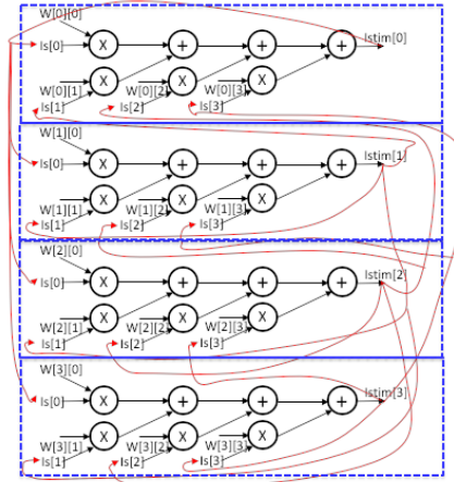
Fig. 9. Multiplication Solution with Global Communication
