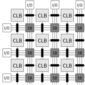
Fig. 1. Traditional FPGA Architecture Fig. 2. Traditional CGRA Architecture
