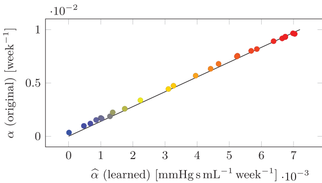
FIGURE 15 Test Case 4: original parameters \alpha^i plotted against the corresponding learned parameters \hat{\alpha}^i for the training individuals ( i = 1, \dots, N_P )
