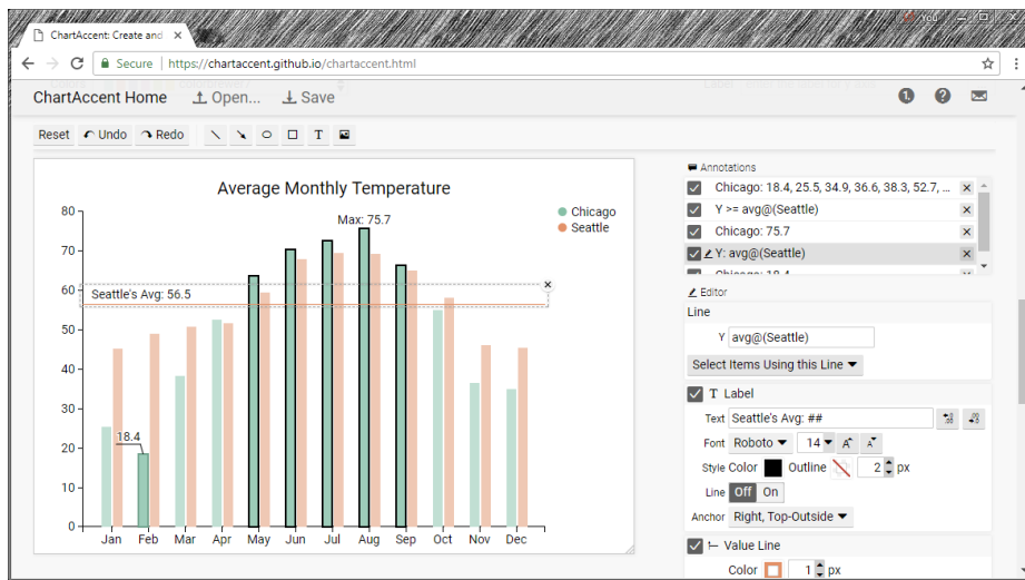
Fig. 2: ChartAccent is a web-based authoring tool that enables people to augment charts using a palette of annotation interactions.
