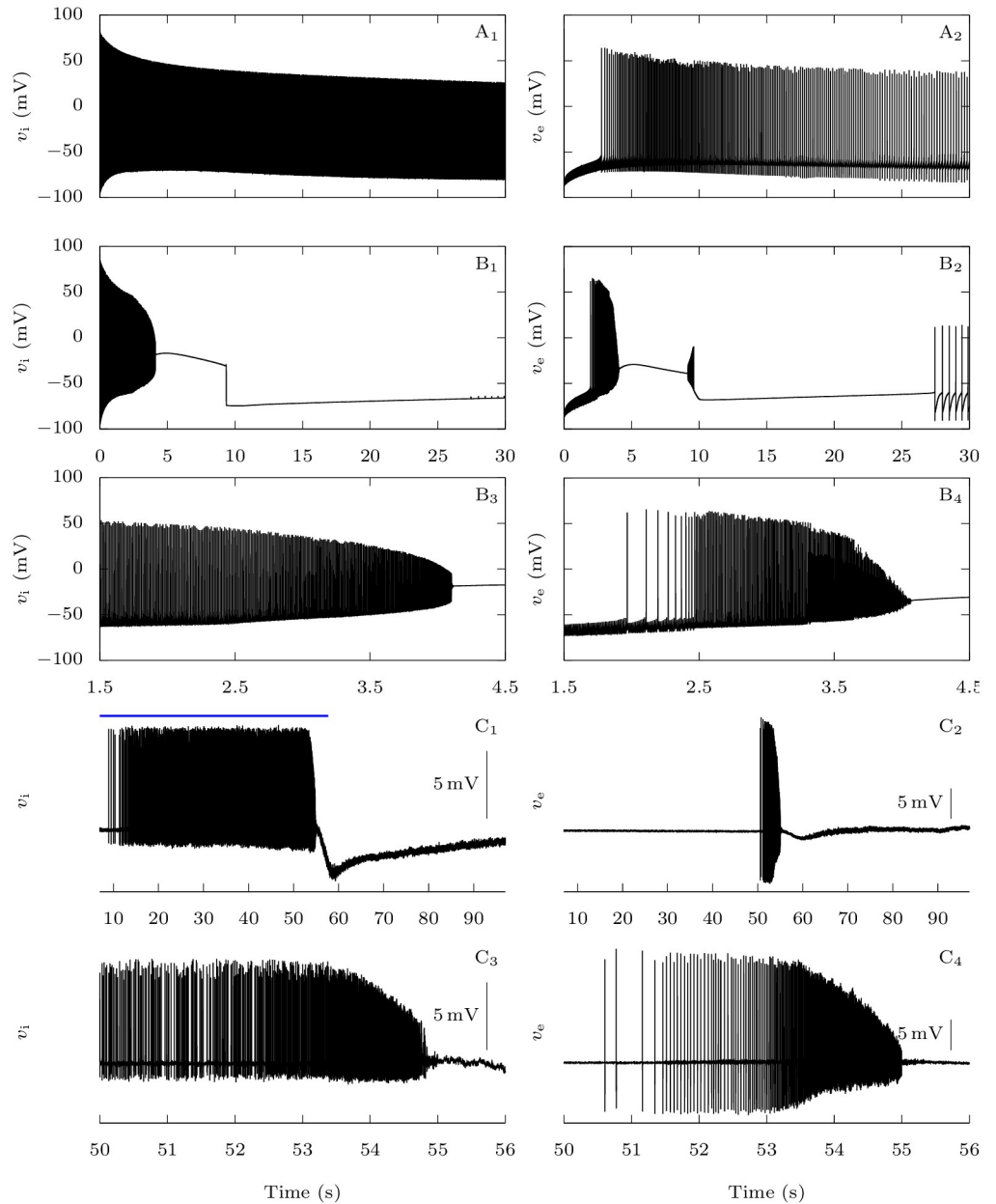
Fig 4. Effect of the FHM-3 mutation on CSD initiation: Representative time traces. A-B: Model simulations. Starting from neurons at rest, similarly to Fig 2, we stimulated them with constant excitatory conductances g_{D,i} = g_{D,e} = 0.3 \text{ mS} \cdot \text{cm}^{-2} for 30 s. A: No persistent sodium current for the GABAergic neuron ( p_{Na,P} = 0\% ). B: Pathological condition ( p_{Na,P} = 15\% ). C: Experimental data. Representative dual juxtacellular-loose patch voltage recordings of a GABAergic interneuron ( C 1 and C 3 ) and a pyramidal neuron ( C 2 and C 4 ) showing the dynamics of the firing at the site of CSD initiation; CSD was induced by spatial optogenetic activation of GABAergic neurons and is the slow negative deflection observable in C 1 and C 2 . The blue bar in C 1 shows the optogenetic stimulation with blue light.
