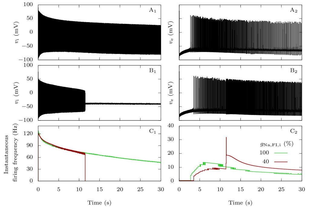
Fig 12. Effect of Na_v1.1 epileptogenic mutations on the firing frequency of the pyramidal neuron. When both neurons are coupled, taking as initial condition the steady-state when there is no external input, we applied external inputs g_{D,i} = g_{D,e} = 0.3 \text{ mS} \cdot \text{cm}^{-2} . We tested both the default parameters, which represent a wild-type GABAergic neuron, and a sodium fast-inactivating maximal conductance g_{Na,FI,i} reduced to 40% of its default value, to model epileptogenic mutations of Na_v1.1 . A: Voltage of the GABAergic ( A_1 ) and pyramidal ( A_2 ) neurons in the wild-type condition. B: Voltage of the GABAergic ( B_1 ) and pyramidal ( B_2 ) neurons with the epileptogenic mutation. C: Instantaneous firing frequency of the GABAergic ( C_1 ) and pyramidal ( C_2 ) neurons in the two conditions.
