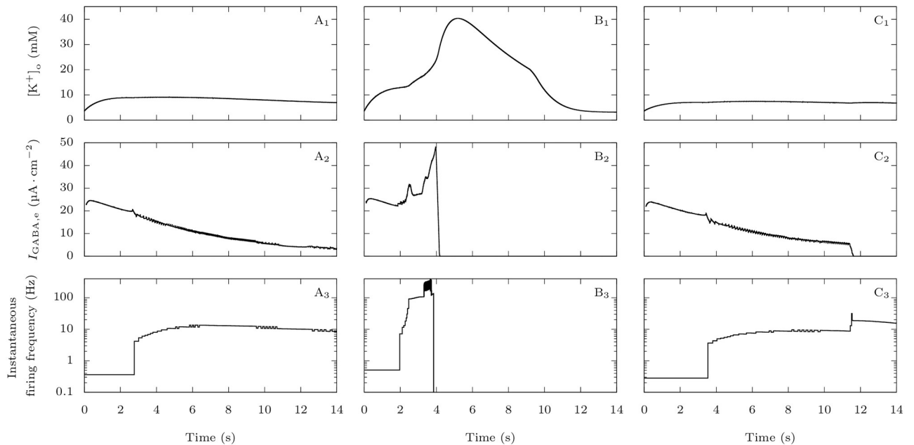
Fig 13. Comparison of migraine and epilepsy scenarios regarding extracellular potassium and GABAergic inhibition. Plots of the extracellular potassium concentration (upper row), GABAergic neuron's inhibitory current on the pyramidal neuron (second row) and pyramidal neuron's firing frequency (bottom row) corresponding to the simulations displayed in Figs 4 and 12. For better readability, we averaged the GABAergic currents on a running window of 200 ms. We show the pyramidal neuron's firing frequency with a logarithmic scale. A: Control condition: default parameter values. B: Migraine condition: percentage of sodium voltage-gated conductance corresponding to persistent current p_{\text{Na,P}} = 15\% . C: Epilepsy condition: sodium fast-inactivating maximal conductance reduced to 40% of its default value.
