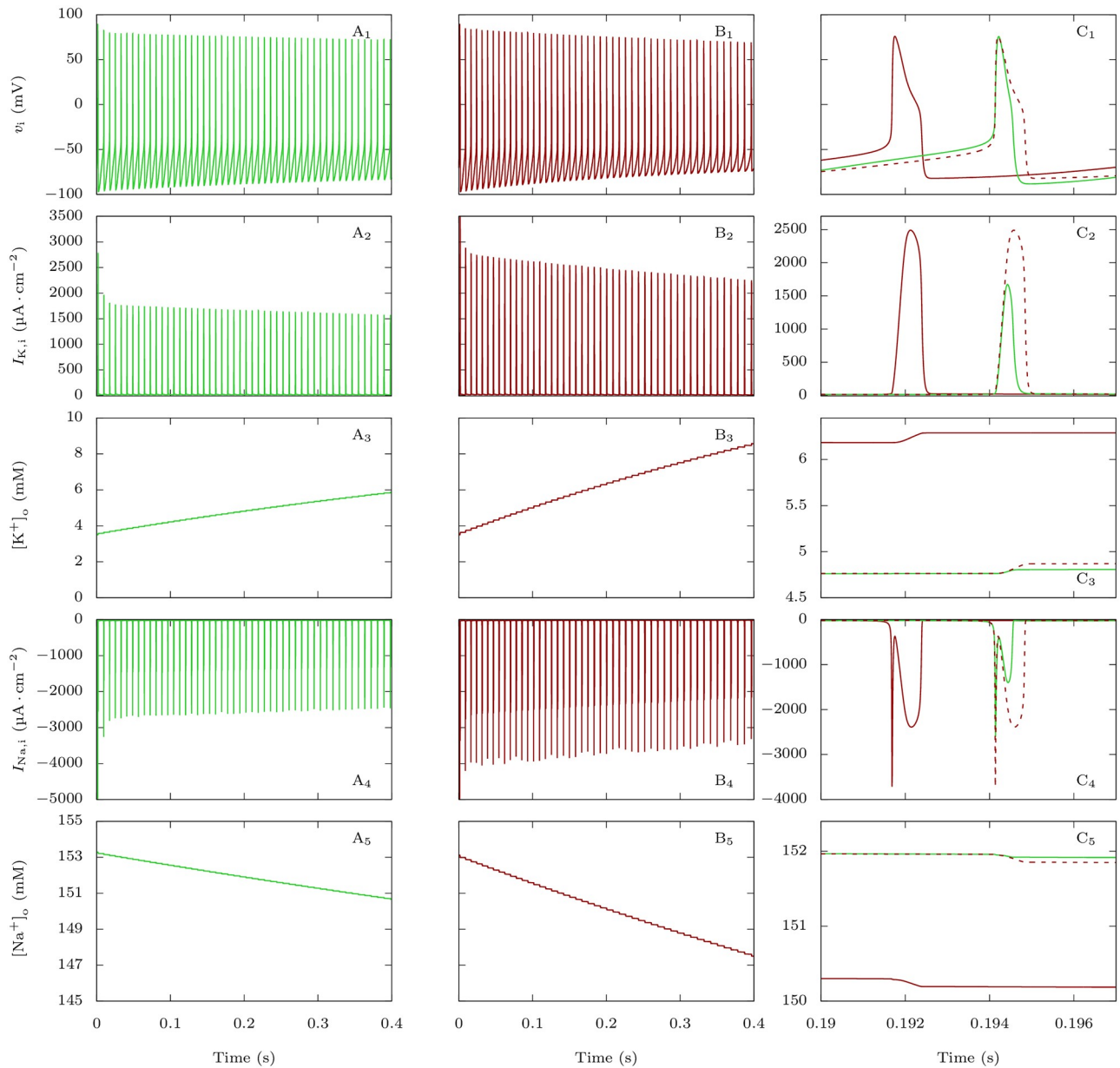
Fig 3. Effect of FHM-3 mutations on the firing and action currents of the GABAergic neuron, and correlation with the dynamics of [K^+]_o and [Na^+]_o . Plots of the voltage (action potentials; upper row), total potassium current (second row), extracellular potassium concentration (third row), total sodium current (fourth row) and extracellular sodium concentration (bottom row) corresponding to simulations displayed in Fig 2, for the condition in which g_{D,i} = 0.3 \text{ mS} \cdot \text{cm}^{-2} . A: No persistent sodium current: p_{Na,P} = 0\% . B: p_{Na,P} = 20\% . C: Zoom showing the 25 th action potential of A (in green) and B (in red). The dashed lines are the curves obtained with p_{Na,P} = 20\% shifted to allow a better comparison with the curves obtained with p_{Na,P} = 0\% .
