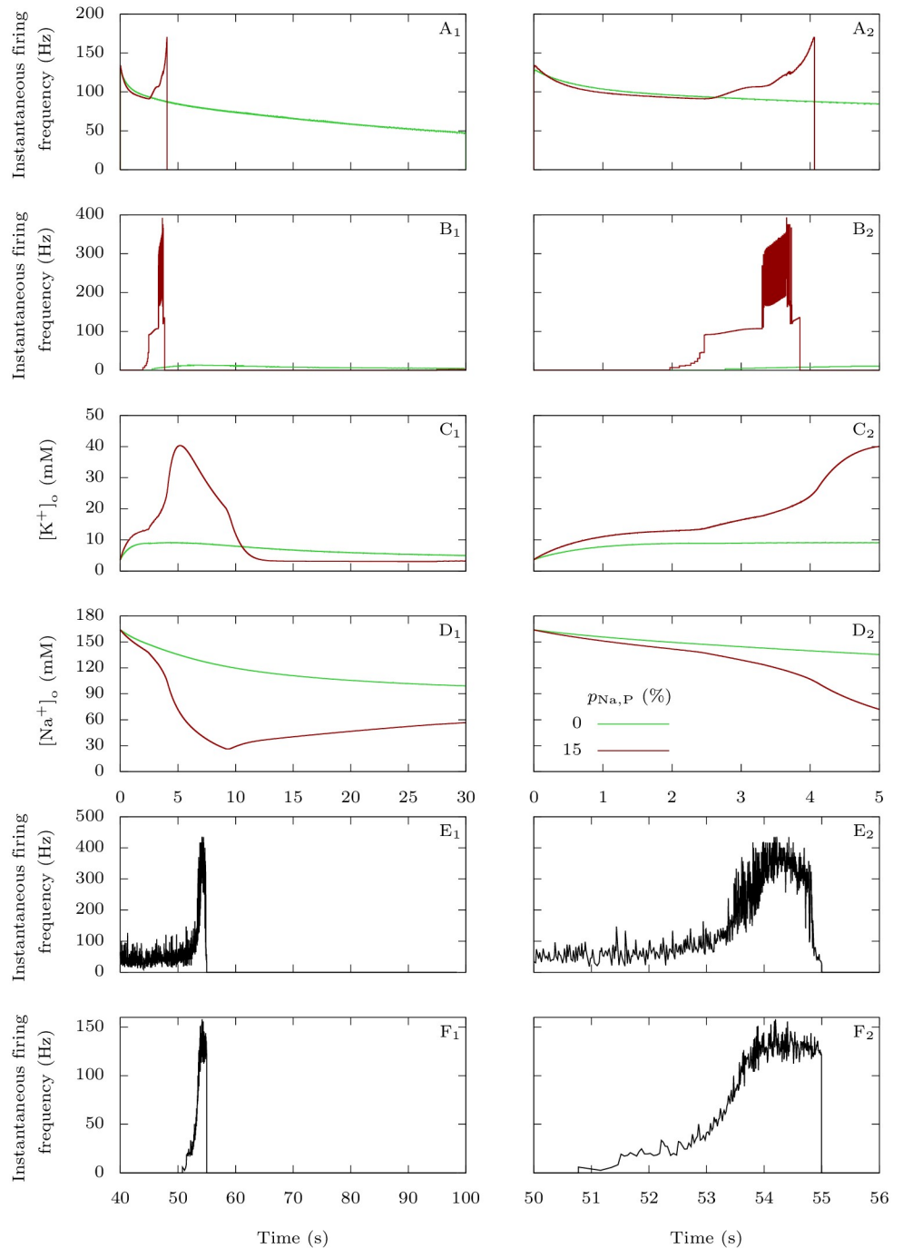
Fig 5. Behavior of the firing frequency and of the extracellular ion concentrations before the onset of CSD. A-D: Model simulations. For the first 5 s of the simulations presented in Fig 4, we compared the pathological situation ( p_{Na,P} = 15\% ) with the physiological one ( p_{Na,P} = 0\% ). A: Instantaneous firing frequency, i.e. inverse of the interspike interval, for the GABAergic neuron. B: Instantaneous firing frequency for the pyramidal neuron. C: Extracellular potassium concentration. D: Extracellular sodium concentration. E-F: Experimental data. E: Instantaneous firing frequency of the loose patch recording of the GABAergic neuron shown in Fig 4C 1 and 4C 3 . F: Instantaneous firing frequency of the loose patch recording of the pyramidal neuron shown in Fig 4C 2 and 4C 4 . CSD was induced by the optogenetic stimulation of the GABAergic neuron; the two phases in the firing dynamics, with lower and higher frequency respectively, are evident and similar to those observed in the simulation. Although the first phase was longer for GABAergic neurons ( 55.3 \pm 4.5 s, n = 7 ) than for pyramidal neurons ( 1.6 \pm 0.2 s, n = 5 ; p = 0.006 Mann-Whitney test), the second phase had similar duration ( 2.0 \pm 0.2 s for GABAergic neurons; 1.7 \pm 0.3 s for pyramidal neurons; p = 0.28 , Mann-Whitney test) and firing frequency was not significantly different (mean instantaneous firing frequency in the
