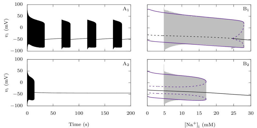
Fig 11. Effect of \text{Na}_v1.1 epileptogenic mutations on the GABAergic neuron bifurcation structure. We considered the intracellular sodium concentration as a slow variable and we studied the corresponding fast subsystem where this concentration is a parameter. We focused here on the case where g_{D,i} = 0.3 \text{ mS} \cdot \text{cm}^{-2} . A: Voltage trace of the full system starting from a neuron at rest, for the default parameter values ( A 1 ) or when the fast-inactivating sodium maximal conductance is reduced to 40% of its default value ( A 2 ). B: Trajectory of A 1 ( B 1 ) or A 2 ( B 2 ), projected onto the ([\text{Na}^+]_i, v_i) plane and bifurcation diagram of the fast subsystem with respect to the intracellular sodium concentration. We represented steady-states with black lines and limit cycles with purple lines.
