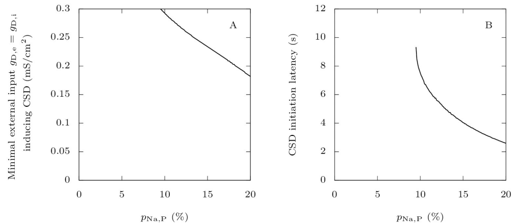
Fig 6. Effect of FHM-3 mutations on CSD initiation. A: We show here how increasing the GABAergic neuron's persistent sodium current influences the minimal external input necessary to induce a depolarization block in the pyramidal neuron, varying p_{\text{Na,P}} from 0 to 20%. We used as external inputs constant excitatory conductances, equal for both neurons, taking values up to g_{D,i} = g_{D,e} = 0.3 \text{ mS} \cdot \text{cm}^{-2} . We considered that beyond these values, inputs would be unrealistically strong, leading to a response of the model that would not be interpretable. Again, we chose as initial condition the steady state when the neurons are not stimulated. We defined a depolarization block by the absence of oscillations of amplitude larger than 5 mV of the voltage for at least half a second, with the additional condition that it must be between -55 \text{ mV} and -20 \text{ mV} at the end of this interval. For each p_{\text{Na,P}} , we estimated the smaller external input for which this criterion is met for the pyramidal neuron with a bisection method. B: Starting from neurons at rest, for given large external inputs g_{D,e} = g_{D,i} = 0.3 \text{ mS} \cdot \text{cm}^{-2} , we computed the time it takes for a CSD to be initiated, if it is initiated at all.
