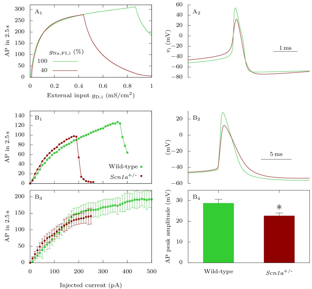
Fig 10. Effect of Na_v1.1 epileptogenic mutations on the firing of GABAergic neurons: Input-output relationship and action potential amplitude. A: Model simulations. We applied to the GABAergic neuron at rest 2.5 s long excitatory external inputs of conductances g_{D,i} for the default parameters (wild-type), or for a reduced sodium fast-inactivating maximal conductance g_{Na,FI,i} (epileptogenic mutations). A 1 : Number of action potentials. A 2 : Representative action potentials, for g_{D,i} = 0.3 \text{ mS} \cdot \text{cm}^{-2} . B: Experimental data. B 1 : Representative fast spiking neurons recorded in cortical slices from Scn1a^{+/-} mice and wild type littermates, selected for having similar input-output curves with lower injected current, showing that the Scn1a^{+/-} neuron was more prone to depolarization block (sharp decrease of action potential number). B 2 : Comparison of the first suprathreshold action potential recorded in the neurons selected for panel B1. B 3 : Mean input-output relationships for fast spiking neurons recorded from Scn1a^{+/-} ( n = 7 ) and wild type littermates ( n = 7 ), the number of elicited action potentials was not different, but depolarization block was induced with lower depolarizing current (the traces in which there was depolarization block were excluded, to avoid the influence of depolarization block in the evaluation of the number of action potentials elicited with larger depolarizing currents). B 4 : Mean peak amplitude (absolute value) of the first suprathreshold action potential for fast spiking neurons recorded from Scn1a^{+/-} ( 22.6 \pm 1.5 \text{ mV} , n = 7 ) and wild type littermates ( 28.7 \pm 2.0 \text{ mV} , n = 7 ); p = 0.044 Mann-Whitney test. * p < 0.05 .
