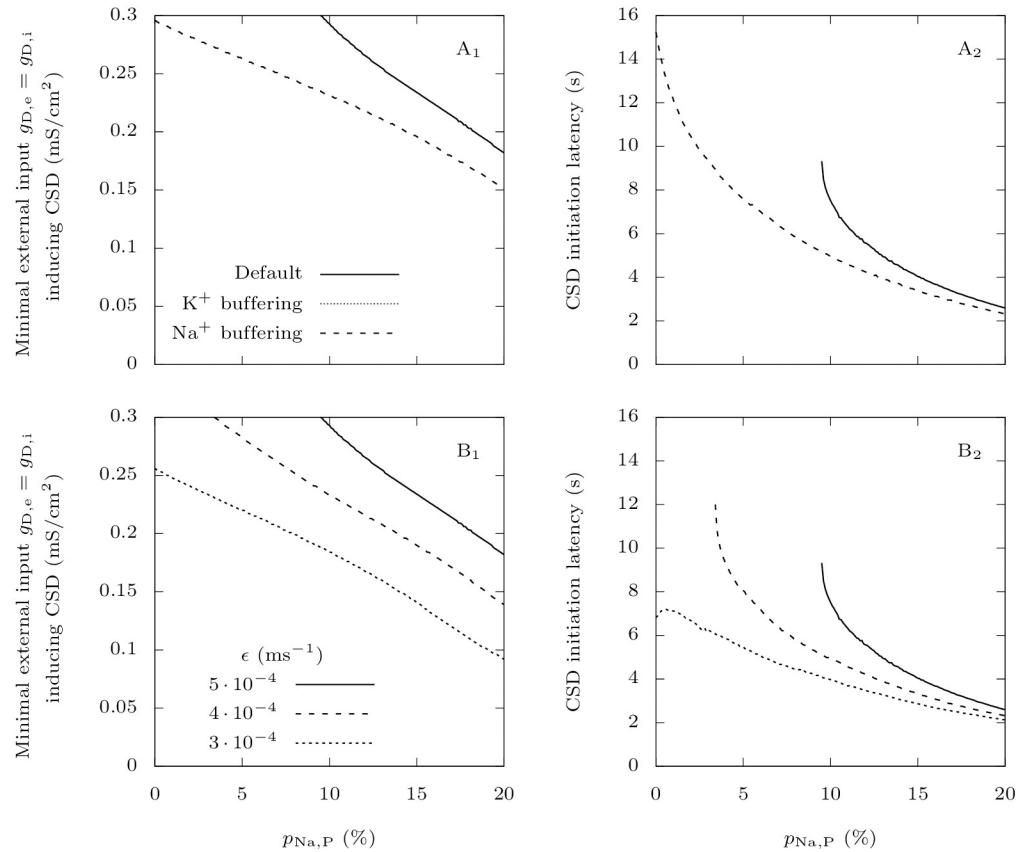
Fig 8. The roles of extracellular ions in CSD initiation. Similarly to Fig 6, we show in the left panel the minimal external input necessary to induce a depolarization block in the pyramidal neuron, and in the right panel the latency to CSD. A: We tested the effect of keeping either extracellular potassium or sodium approximately constant using the same method as for Fig 7. B: We tested the effect of reducing the extracellular potassium diffusion rate. The default value of this parameter is \epsilon = 5 \cdot 10^{-4} \text{ ms}^{-1} .
