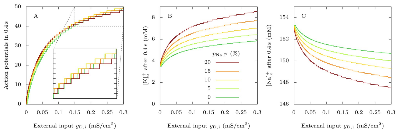
Fig 2. Effect of FHM-3 mutations on the firing properties of the GABAergic neuron. For different values of p_{\text{Na,P}} (defined in Section 2.2.6), which we increase to model FHM-3 mutations, we applied to the GABAergic neuron 0.4 s long excitatory external inputs of conductances g_{D,i} . For each p_{\text{Na,P}} value, we took as initial condition the steady state in the absence of external input, i.e. when g_{D,i} = 0 \text{ mS} \cdot \text{cm}^{-2} . A: Number of action potentials, considered as overshooting spikes (i.e. exceeding 0 mV of peak membrane potential). B: Extracellular potassium concentration at the end of the 0.4 s long simulations. C: Extracellular sodium concentration at the end of the 0.4 s long simulations.
