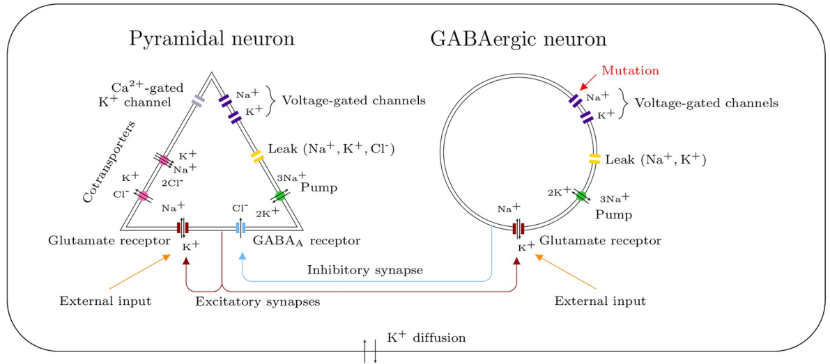
Fig 1. Schematic representation of the model. Consider a pair of interconnected neurons in a closed volume. We modeled a GABAergic synapse from the GABAergic neuron to the pyramidal one, a glutamatergic synapse from the pyramidal neuron to the GABAergic one and a glutamatergic autapse from the pyramidal neuron to itself. The ion transport mechanisms represented here generate transmembrane ionic currents, which modify the membrane potentials of the neurons and the ion concentrations in the different compartments. The diffusion of extracellular potassium takes into account both passive diffusion and glial buffering. We modeled external stimuli, which reflect the activity of the surrounding network or mimic experimental depolarizations, with glutamate inputs on the glutamatergic receptors. The implementation of Na_v1.1 's genetic mutations affects only the GABAergic neuron.
