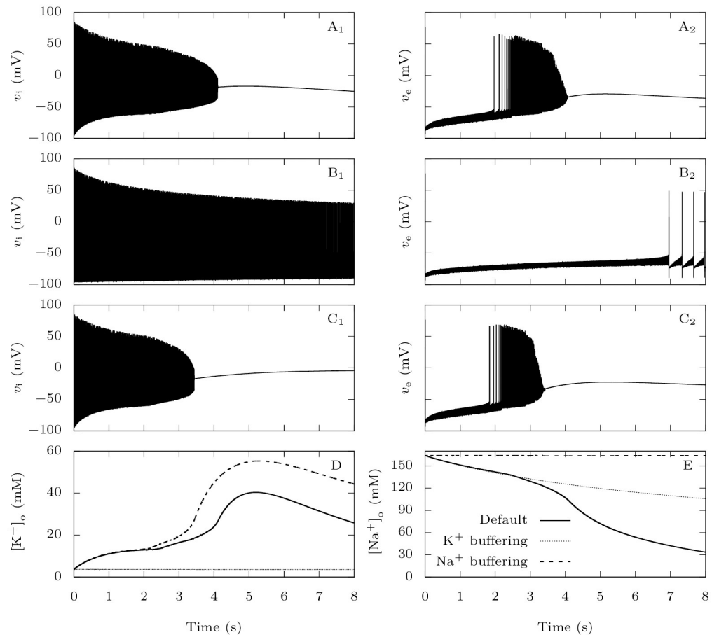
Fig 7. The roles of extracellular ions in CSD initiation: Representative time traces. When \text{Na}_v1.1 carries a FHM-3 mutation, modeled by p_{\text{Na},P} = 15\% , we tested the effect of keeping either extracellular potassium or sodium constant using unrealistically high diffusion rates. We depolarized the neurons at rest with constant excitatory conductances g_{D,i} = g_{D,e} = 0.3 \text{ mS} \cdot \text{cm}^{-2} for 30 s. A: Voltage traces for the default parameters. B: Voltage traces when \epsilon = 0.1 \text{ ms}^{-1} to simulate a strong buffering of extracellular potassium. C: Voltage traces when there is a strong buffering of extracellular sodium. To implement it, we introduced the diffusion term I_{\text{diff,Na}} = \epsilon_{\text{Na}}([\text{Na}^+]_o - \text{Na}_{\text{bath}}) in the equation for extracellular sodium, with \epsilon_{\text{Na}} = 0.1 \text{ ms}^{-1} and \text{Na}_{\text{bath}} equal to the steady-state extracellular sodium in the absence of external input. D: [\text{K}^+]_o traces in the cases described in A-C. E: [\text{Na}^+]_o traces in the cases described in A-C.
