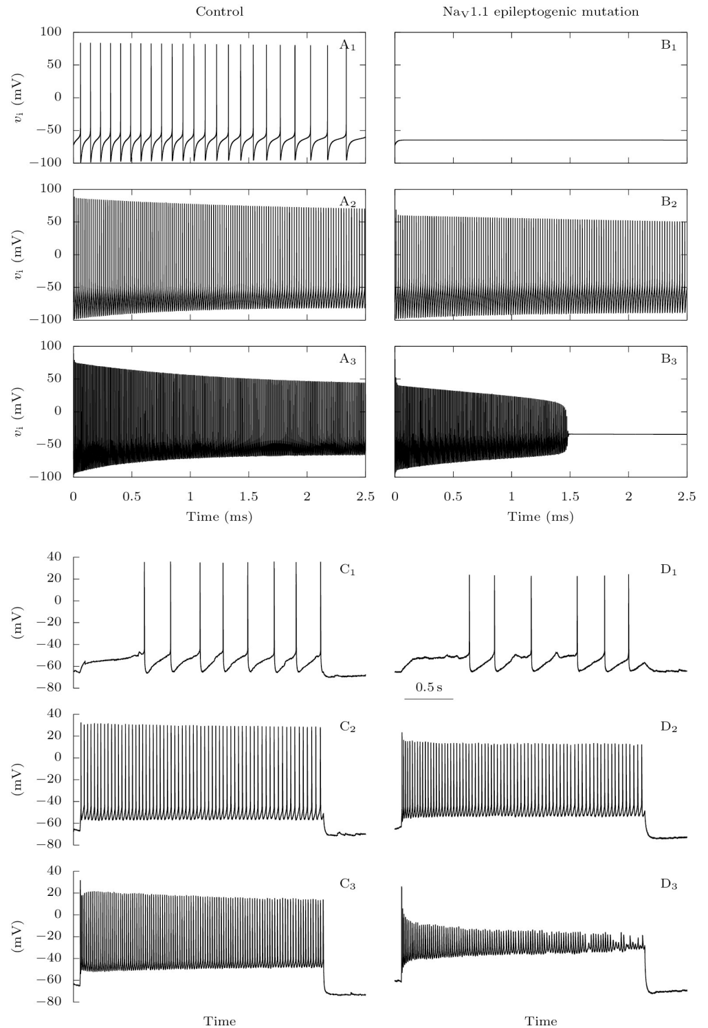
Fig 9. Effect of Na_v1.1 epileptogenic mutations on the firing of GABAergic neurons: Representative traces. A-B: Model simulations. We depolarized the GABAergic neuron at rest with constant excitatory conductances g_{D,i} = 0.0075 (A 1 , B 1 ), g_{D,i} = 0.05 (A 2 , B 2 ) or g_{D,i} = 0.5 \text{ mS} \cdot \text{cm}^{-2} (A 3 , B 3 ), for the default parameters (A: control condition), or when the sodium fast-inactivating maximal conductance is reduced to 40% of its default value (B: Na_v1.1 epileptogenic mutation). C-D: Experimental data. Action potential discharges elicited in a fast spiking GABAergic layer 2-3 cortical neuron from a wild type mouse (C) or a Scn1a^{+/-} mouse (D), injecting depolarizing current steps of 10 pA (C 1 , D 1 ), 100 pA (C 2 , D 2 ) or 260 pA (C 3 , D 3 ).
