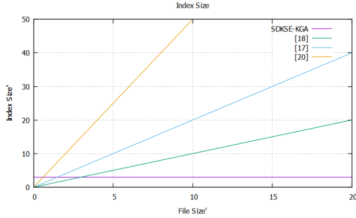
Fig. 3: Index Size
