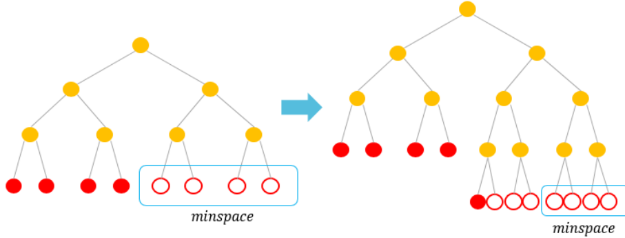
Fig. 2: Grow Tree
