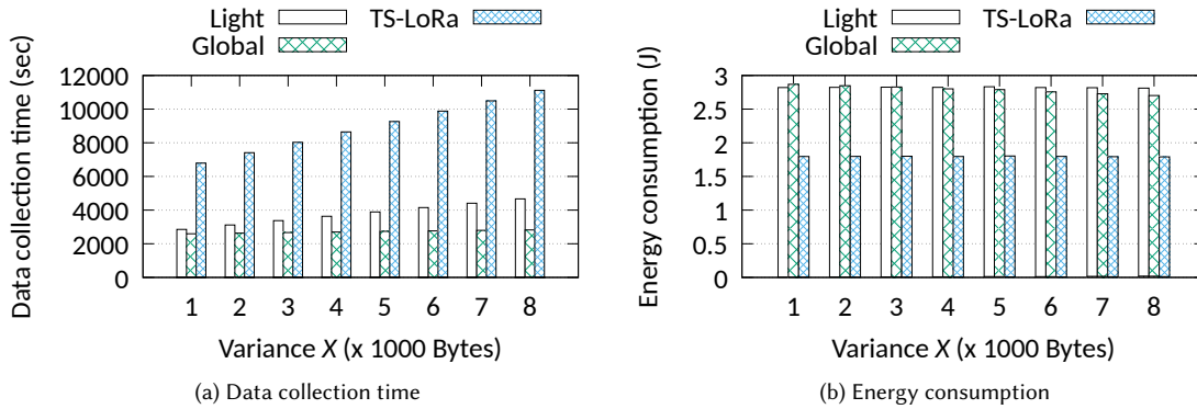
Fig. 6. Data collection time and energy consumption for variable data sizes.
