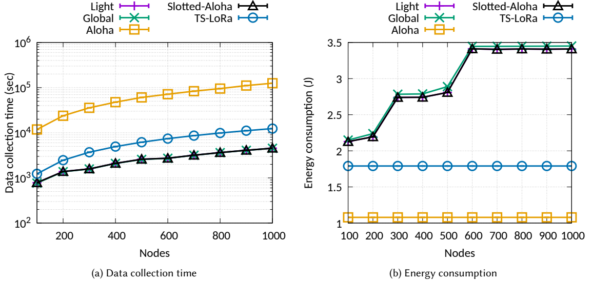
Fig. 5. Data collection time and energy consumption for a scenario with fixed data size.
