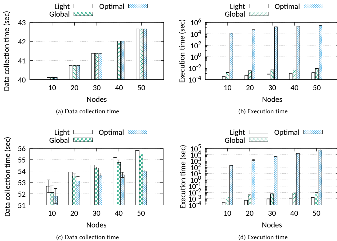
Fig. 4. Comparison with the optimal for a scenario with fixed data size (upper) and variable data size (lower).
