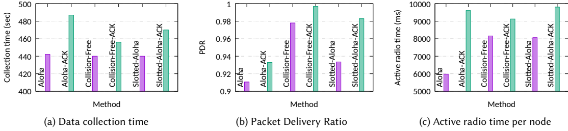
Fig. 10. Experiment with 10 nodes: Data collection time, Packet Delivery Ratio, and active radio time with and without retransmissions (CF: Collision-Free approaches, S-Aloha: Slotted-Aloha, -ACK: the corresponding approach with retransmissions).
