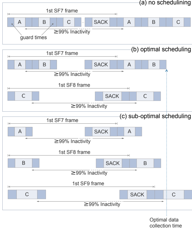
Fig. 3. Different slot and SF allocations of three transmissions with the same packet length and SF7: (a) no extra scheduling is performed. All nodes are serially placed in slots of the SF7 frame one after the other. This is a sub-optimal solution in terms of data collection time. (b) Node C is switched to SF8 frame. This is the optimal solution since it results to minimum data collection time. (c) Node B is switched to SF8 frame and node C to SF9 frame. This is also a sub-optimal solution.
