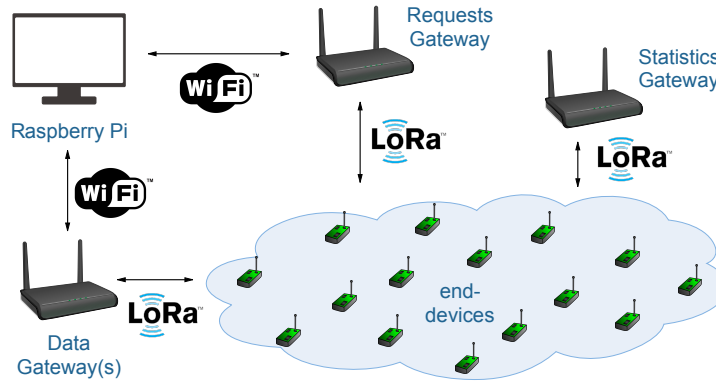
Fig. 9. Network architecture of the experiments.
