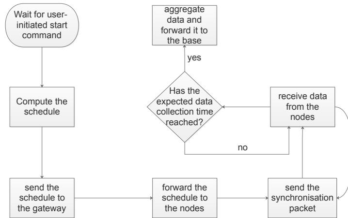
Fig. 8. Experimental procedure of Base/Gateway.
