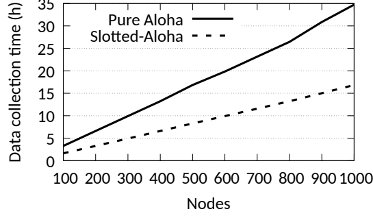
Fig. 2. Theoretical average data collection time ( pkt/\theta ) of an Aloha and Slotted-Aloha LoRa MAC for different node populations, pkt=100 , and 100 Bytes packet size. At least 90% packet success rate of all the nodes is guaranteed.
