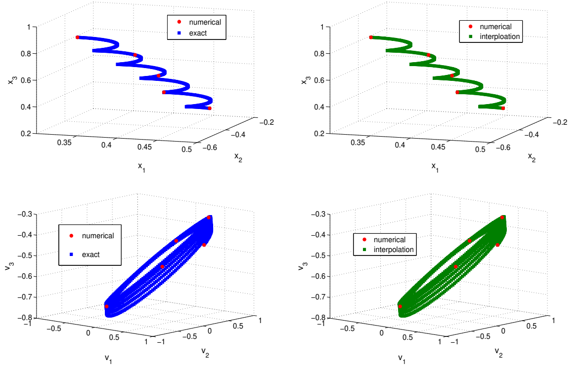
FIGURE 8. Left column: exact trajectory of the particle (blue squares) and the numerical solution of AB-MM with time step \Delta t = 1/4 till t = 1 under \epsilon = 1/2^5 (red dots, ratio \Delta t/\epsilon = 8 ). Right column: the numerical solution under \Delta t = 1/4 and the fully recovered trajectory with quadratic interpolation at fine mesh.
