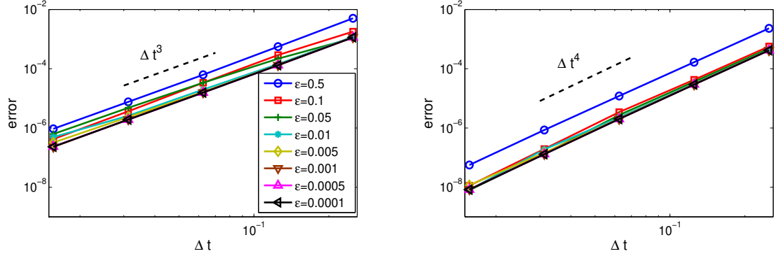
FIGURE 7. Error |\mathbf{x}(t_n) - \mathbf{x}^n|/|\mathbf{x}(t_n)| + |\mathbf{v}(t_n) - \mathbf{v}^n|/|\mathbf{v}(t_n)| as \Delta t for different \epsilon : the 3rd order (left) and the 4th order (right) AB-MM in example 5.2.
