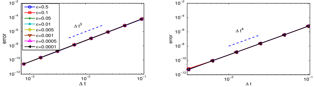
FIGURE 2. Error as \Delta t for different \varepsilon : the 3rd order (left) and the 4th order (right) AB-MM methods in example 5.1.
