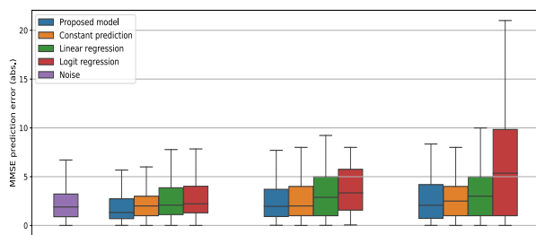
(a) MMSE prediction errors on the AIBL cohort 1.5, 3.0 and 4.5 years ahead.
