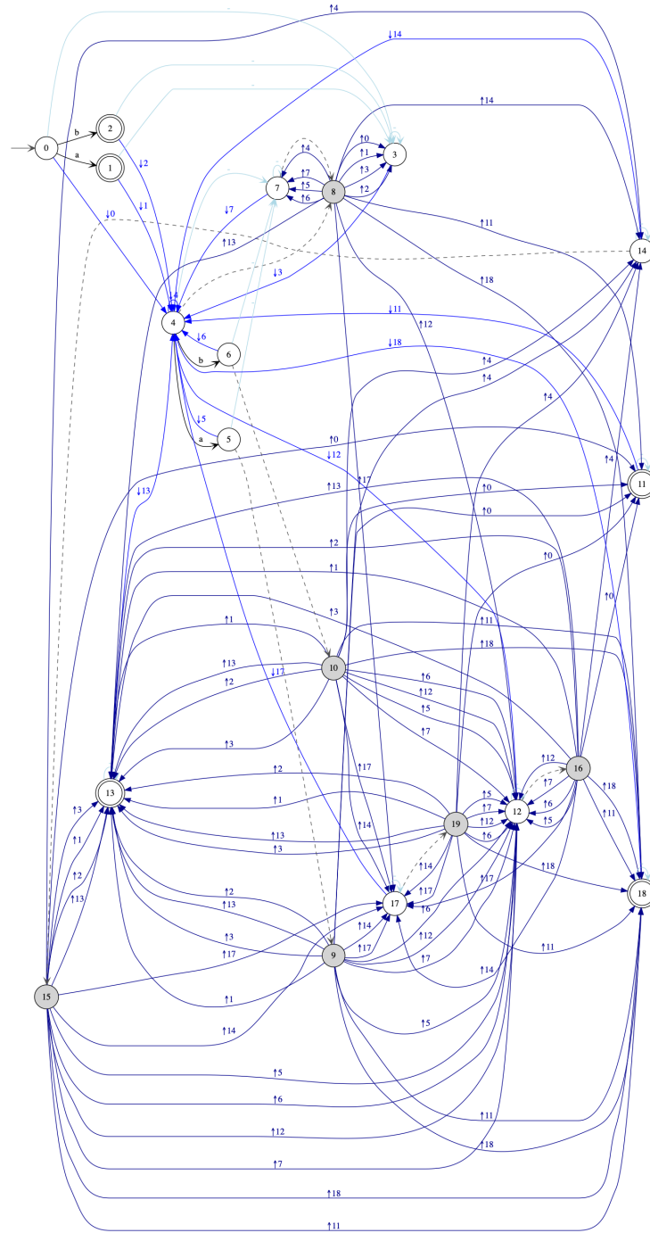
Figure A4. Determinization of NWA from stepwise hedge automaton: \det(nva(\text{step}(ch^*(a + b)))) .
