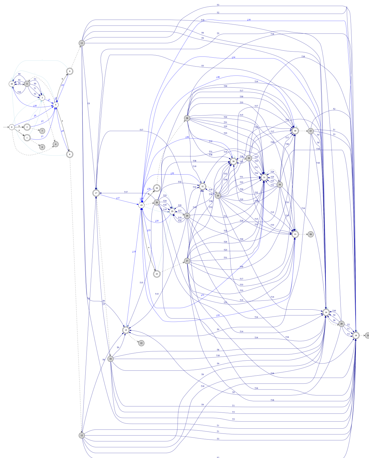
Figure A2. Deterministic NWA: \det(nwa(ch^*(a+b))) .
