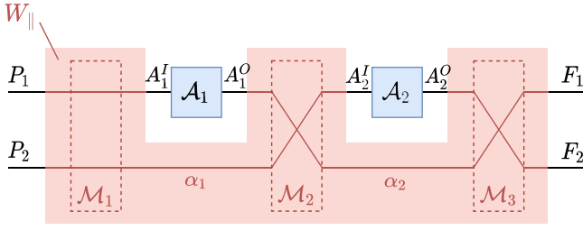
FIG. 6. A QC-FO which applies the CP maps \mathcal{A}_1 and \mathcal{A}_2 to the respective parts of a bipartite system prepared in \mathcal{H}^{P_1} \otimes \mathcal{H}^{P_2} , and then sends the outputs to \mathcal{H}^{F_1} \otimes \mathcal{H}^{F_2} . The process matrix describing this QC-FO, W_{\parallel} , could also be implemented as a QC-FO compatible with the order \mathcal{A}_2 \prec \mathcal{A}_1 , or directly as a QC-PAR (cf. Appendix C).
