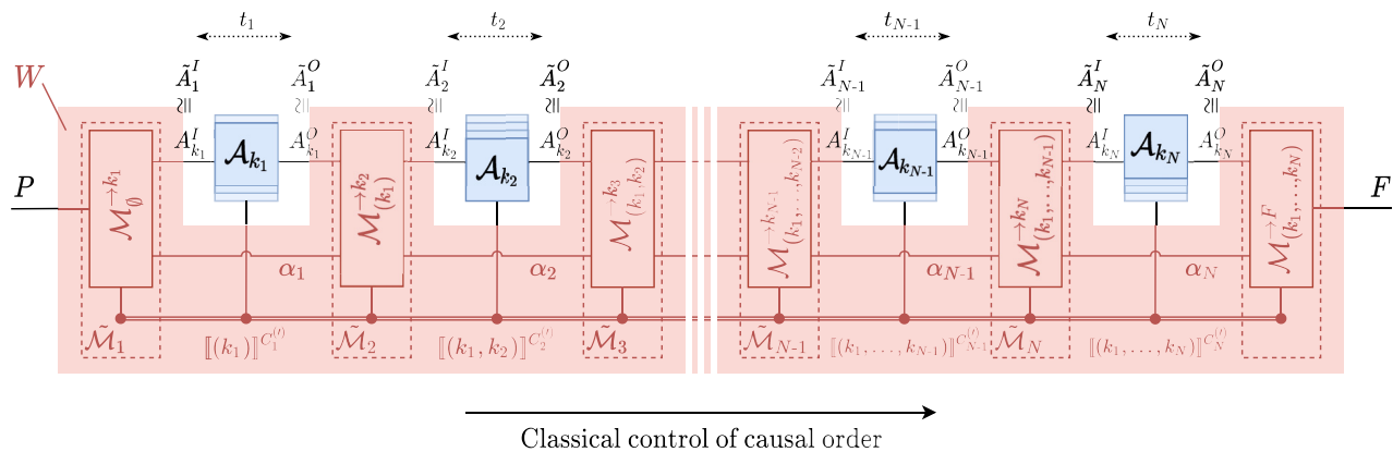
FIG. 9. Another possible representation of a QC-CC, equivalent to Fig. 7. Here we show explicitly the transmission of the information about the causal order, established dynamically and stored on the fly in the states [(k_1, \dots, k_n)]^{(c)} of some control system. The double-stroke lines indicate that this information is classical. This information is used to control which external operation \mathcal{A}_{k_n} is to be applied at each time slot t_n , thus defining the joint operation \tilde{\mathcal{A}}_n of Eq. (35) on the target and control systems. It is also used to control the internal circuit operations \mathcal{M}_{\emptyset}^{\rightarrow k_1} , \mathcal{M}_{(k_1, \dots, k_n)}^{\rightarrow k_{n+1}} , and \mathcal{M}_{(k_1, \dots, k_N)}^{\rightarrow F} , defining the joint operations \tilde{\mathcal{M}}_1 , \tilde{\mathcal{M}}_{n+1} , and \tilde{\mathcal{M}}_N of Eqs. (37)–(39) on the target, ancillary, and control systems.
