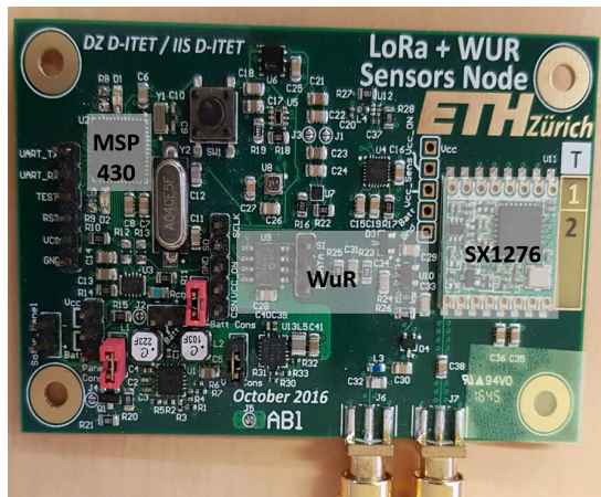
(a) Platform used for experimentations
