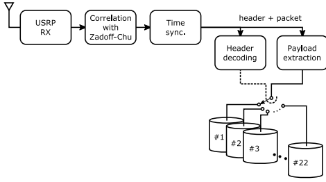
Fig. 6. Reception flowgraph.
