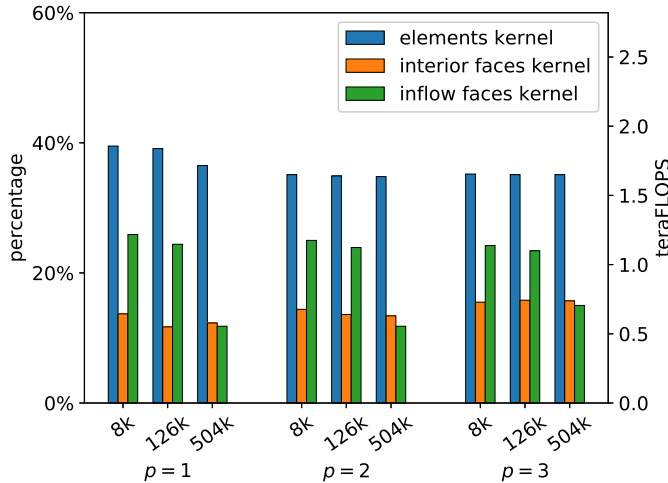
FIG. 10. Double precision performance of the three main kernels on the 3 meshes from Table 4, for p = 1, 2, 3 .
