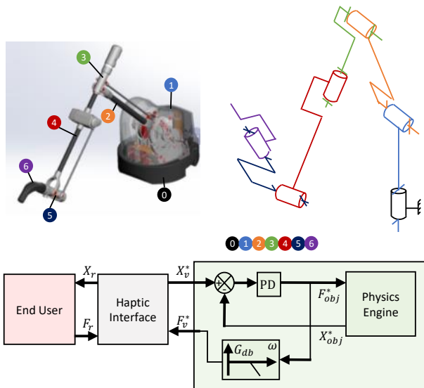
Fig. 1. Top left : Virtuoso6D 3D mock-up. Top right : Kinematic scheme of the HI. Bottom : Detailed haptic interaction. End-user interacted with the haptic display by moving the end-effector X_r . The position of each joint X_v^* was captured, digitalized and sent to the VE. It was coupled to the object scene through a virtual spring-damper because of the admittance control of Rigidbody, the physics engine used. The resulting force F_v^* was low-pass filtered and sent to the HI and used to apply to the end-effector as the force feedback.
